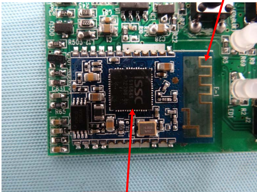
Bluetooth Chip
