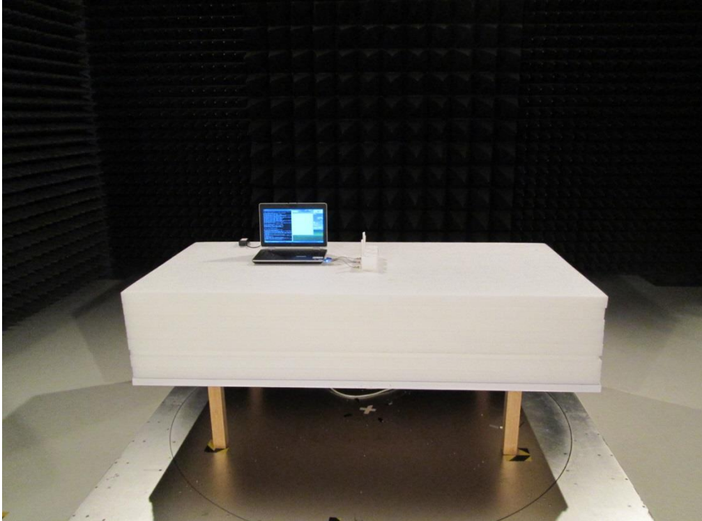
Radiated Test_Ant 1
