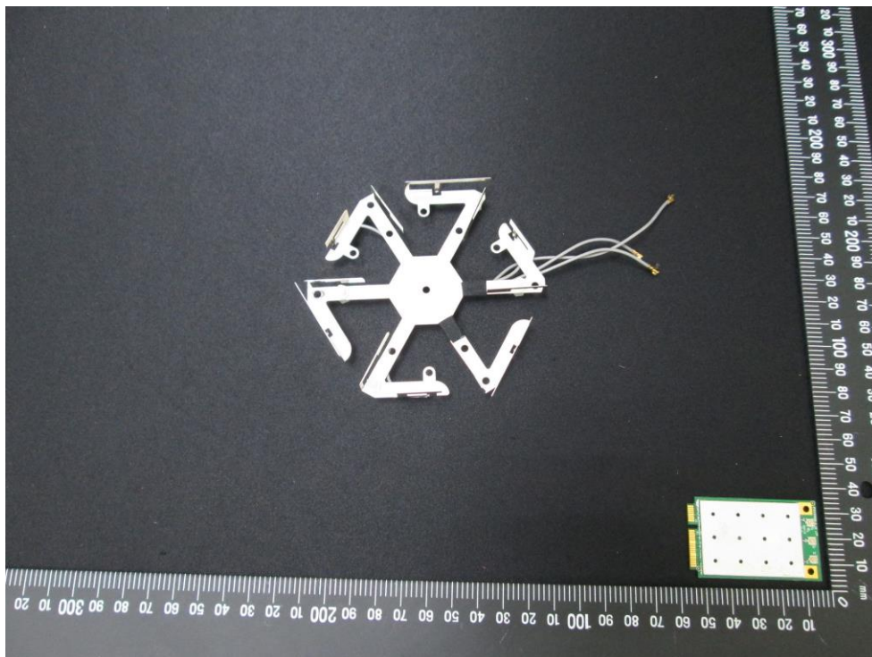
EUT with 6 dBi PIFA Antenna
