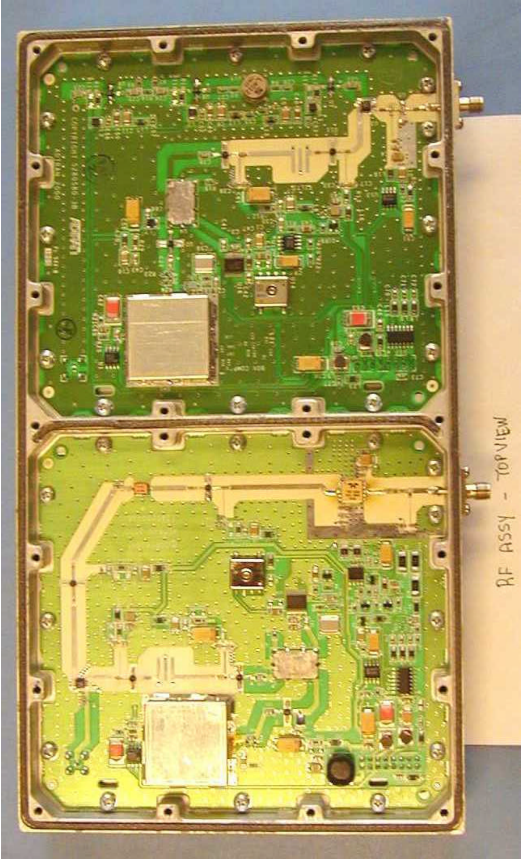
RF Top View
