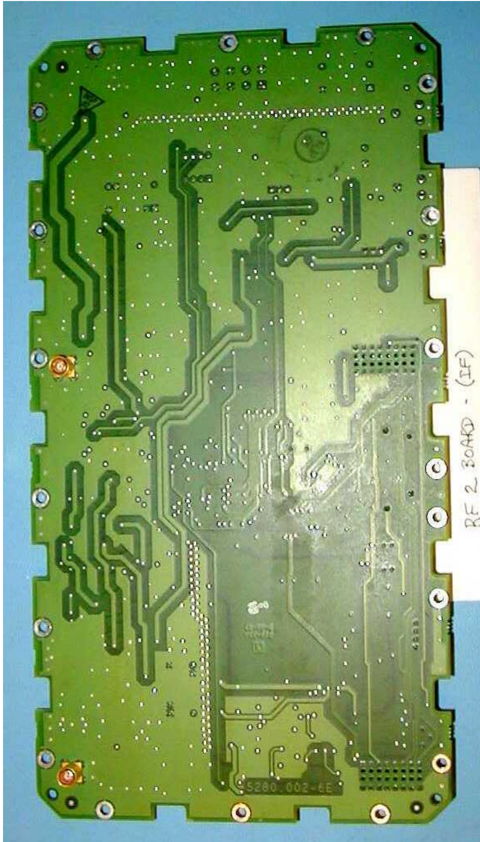
RF PCB, Bottom
