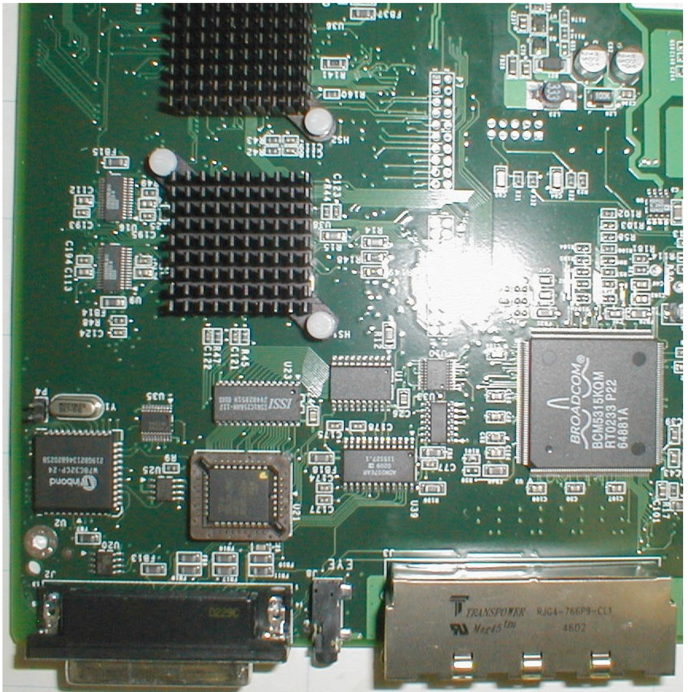
Baseband Board Top, Detail B
