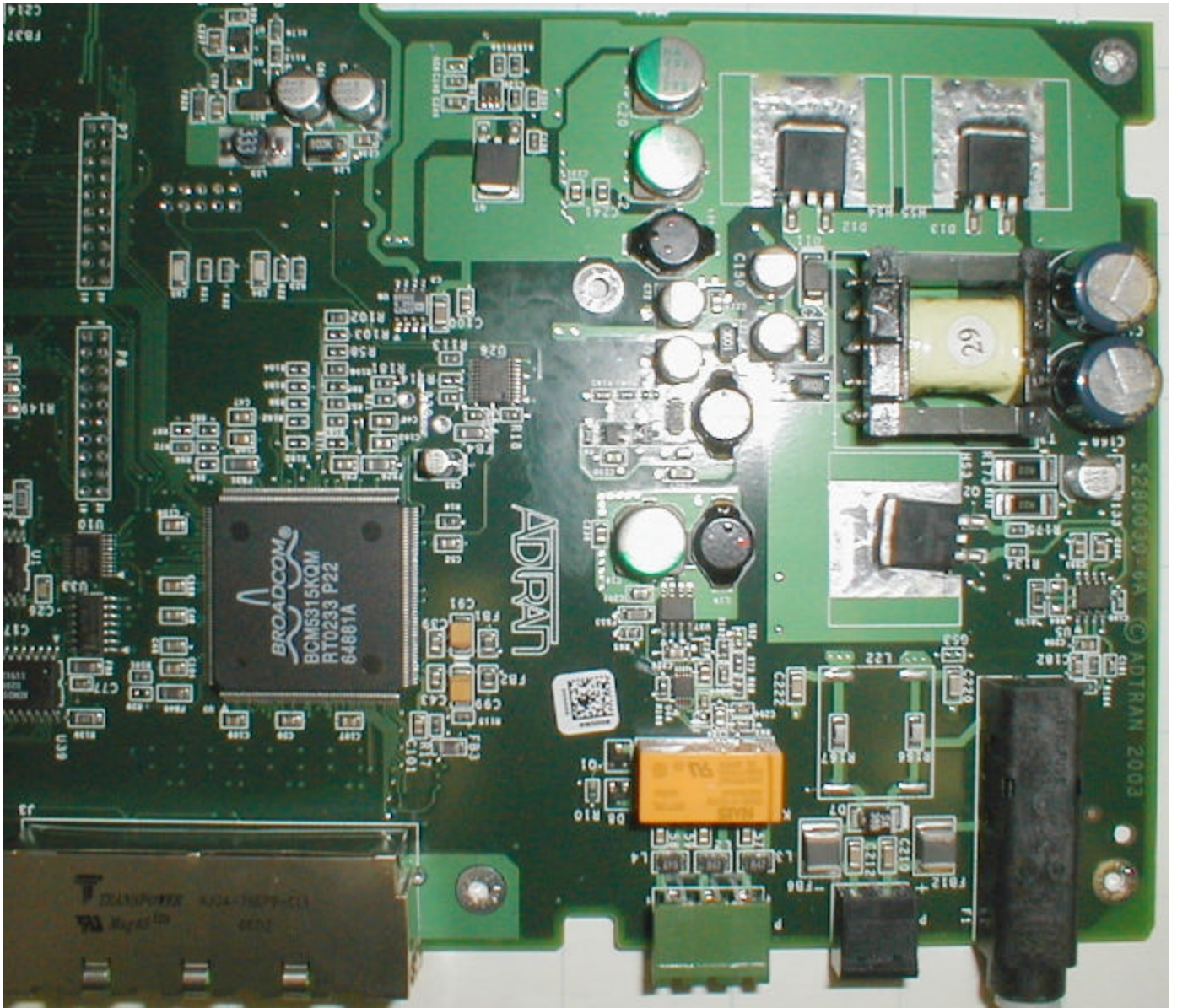
Baseband Board Top, Detail C
