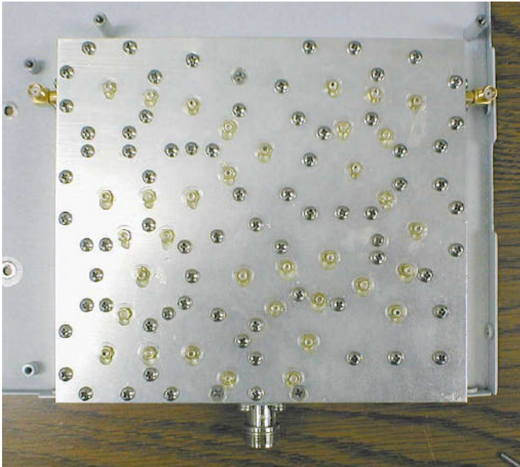
Signal Filter, Top View
