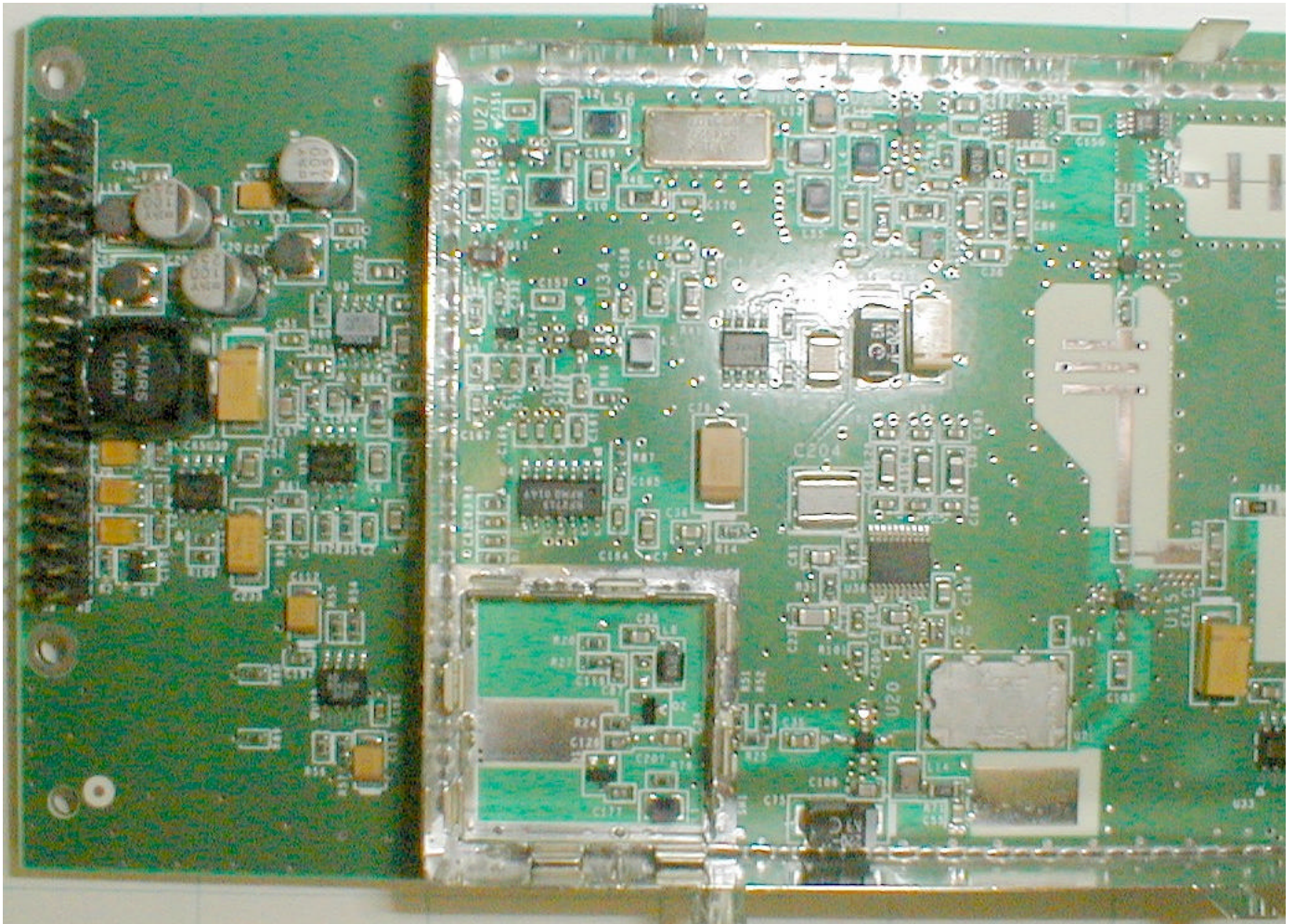
RF Board Bottom Left Detail
