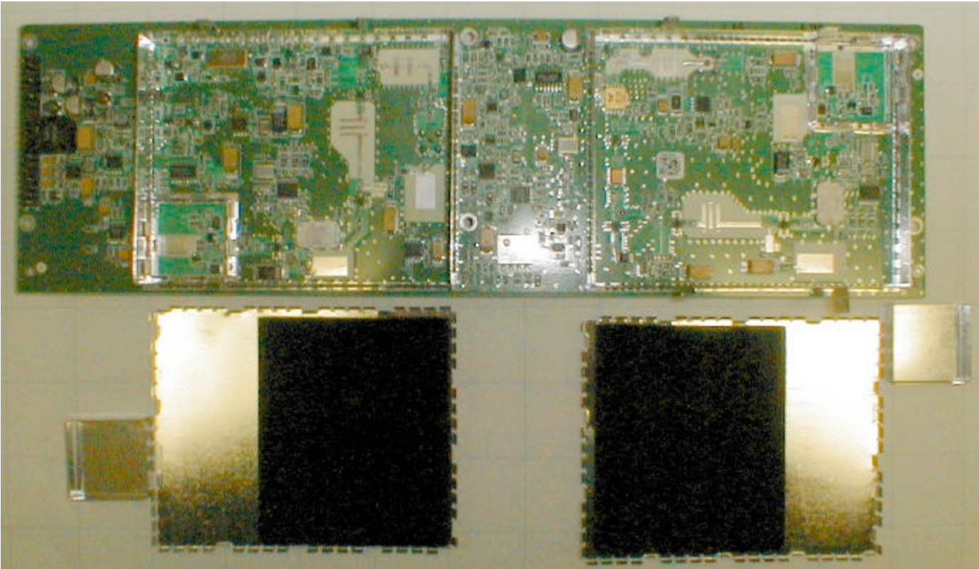
RF Board Bottom Overview Shields Removed
