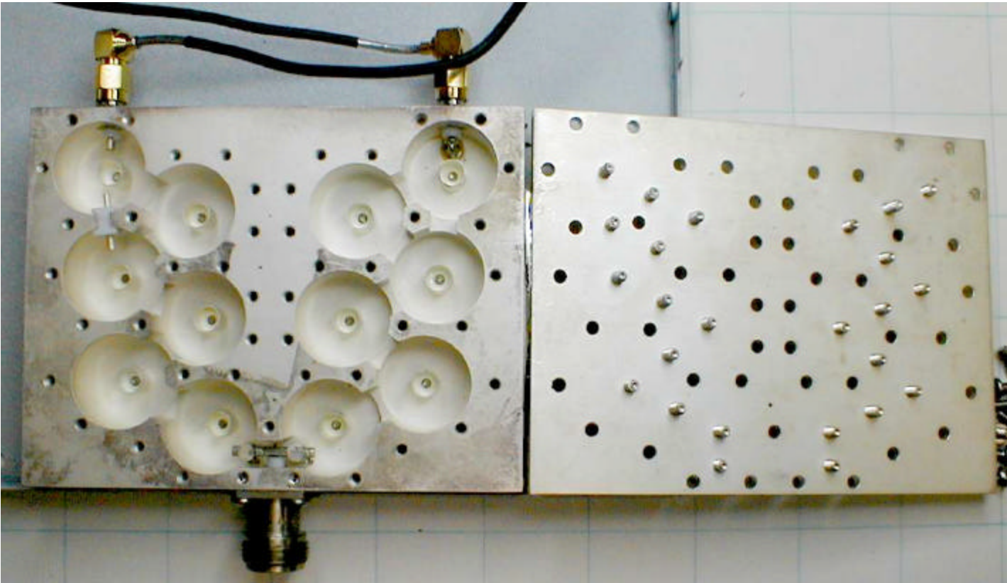
Signal Filter, Internal View
