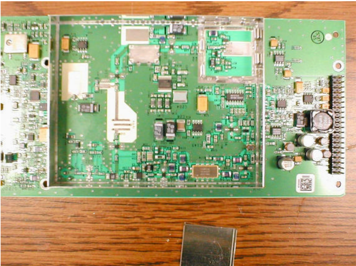
RFC Board, Right Side Detail, Small Shield Removed
