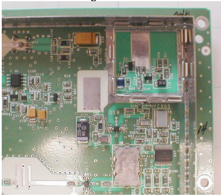
RFC Board Bottom Right Detail, Small Shield Removed
