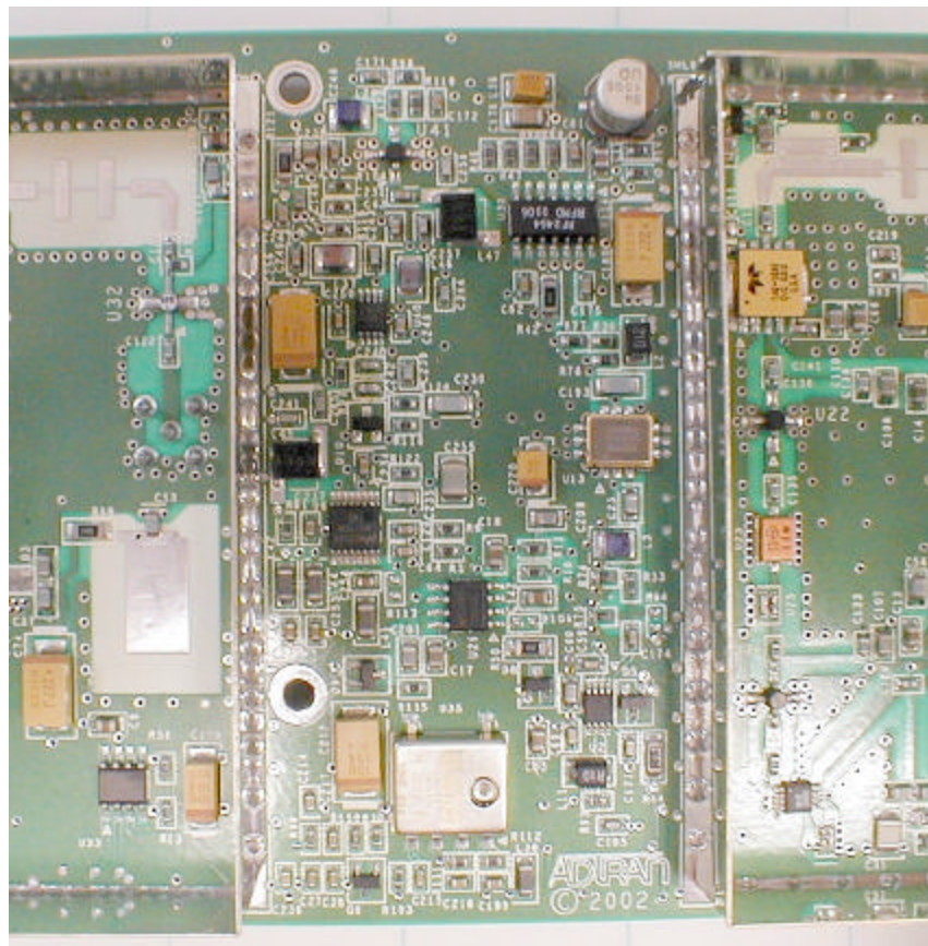
RFC Board Bottom Center
