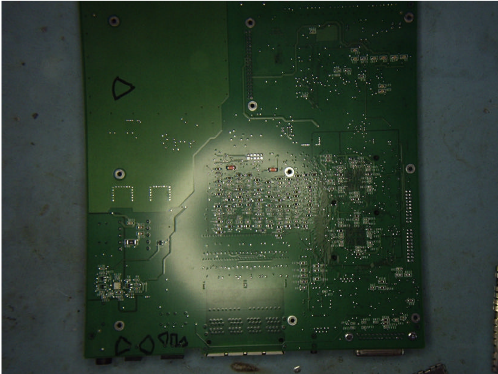
FCC ID: HDCTRC4108L1 Internal Photos - Main Board (Solder Side)
