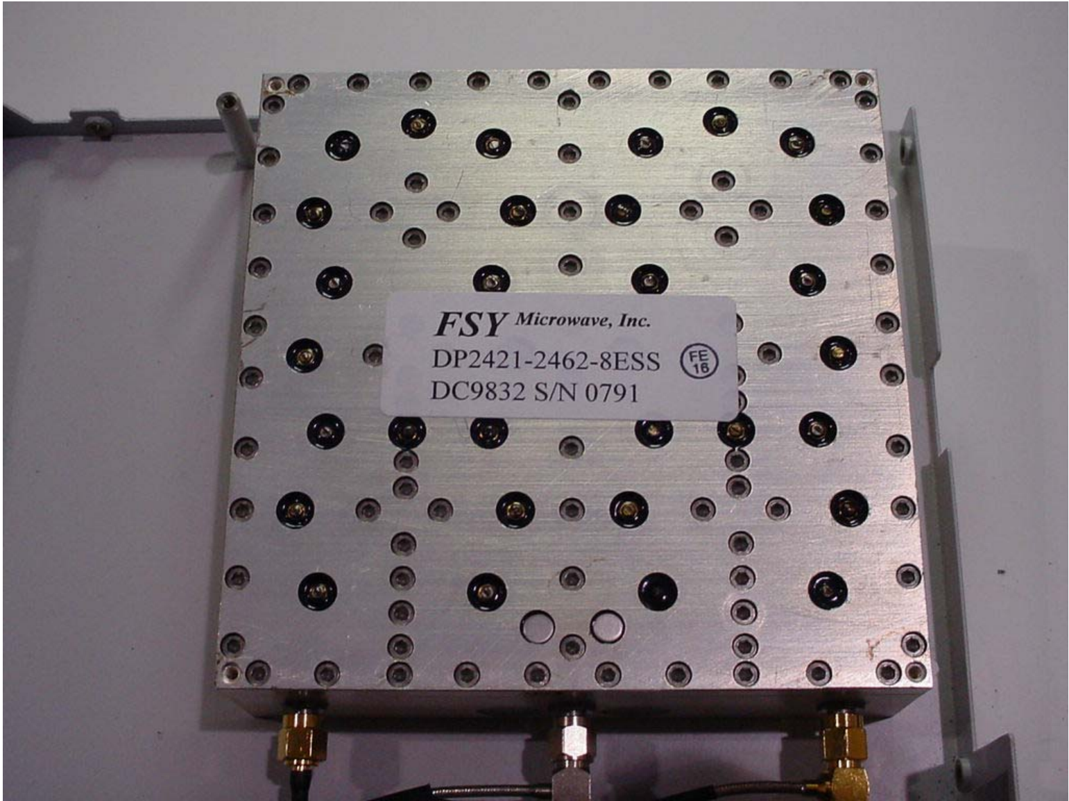
Diplexer
