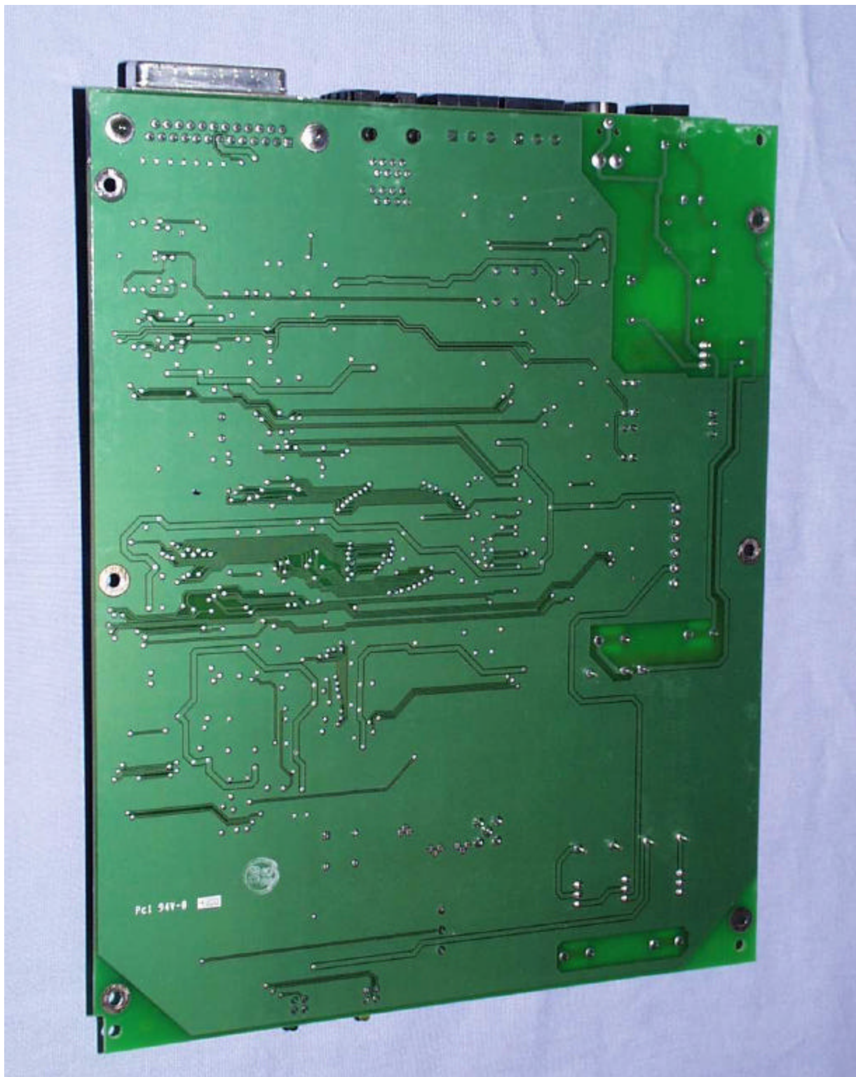
Photograph 2.7 Tracer Monitored Protection Switch Main PCB – Solder Side
