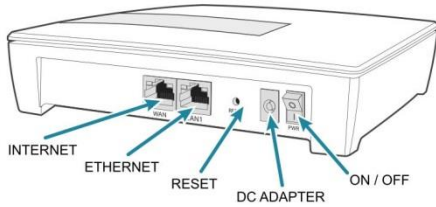
Figure 3. Rear and Side Panel Features
