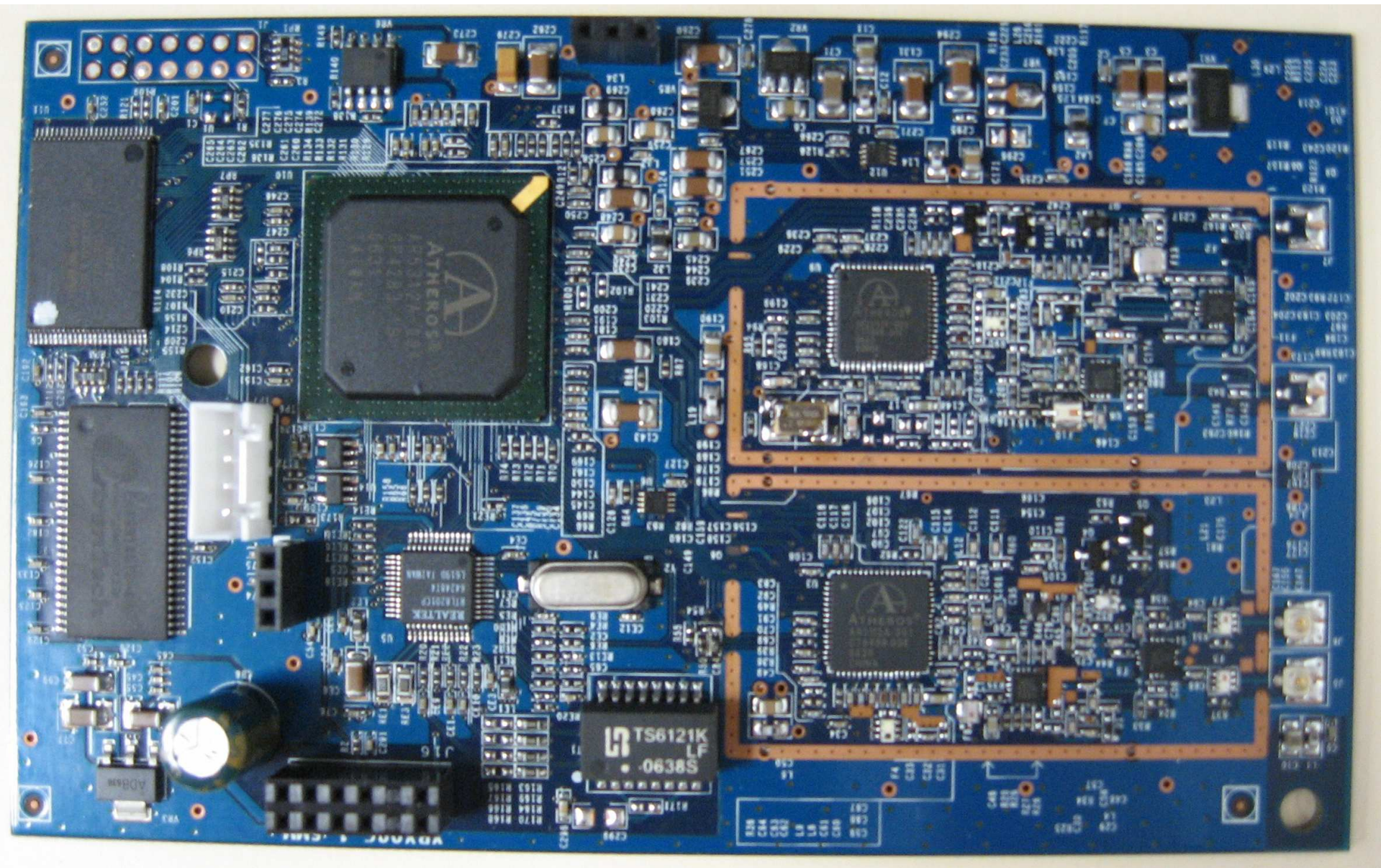
RF Module – Side A with shields removed
