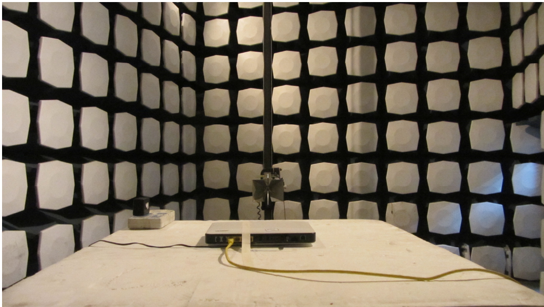
Above 1GHz
