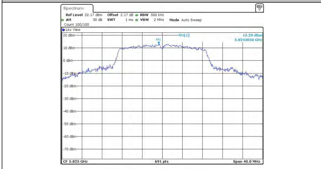
11N20SISO_Ant3_5825
