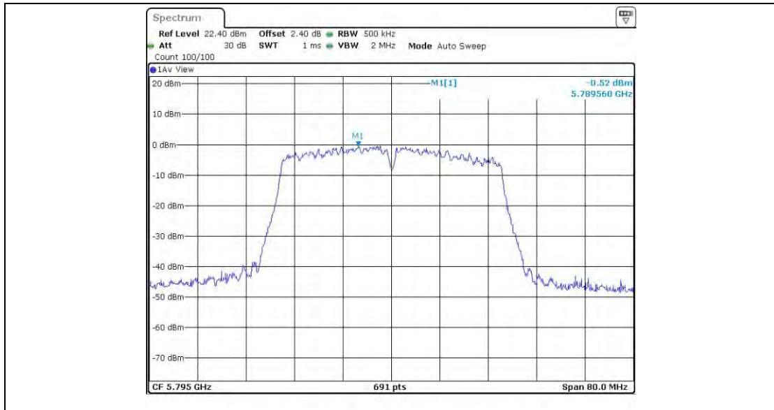
11N40BF_Ant4_5795
