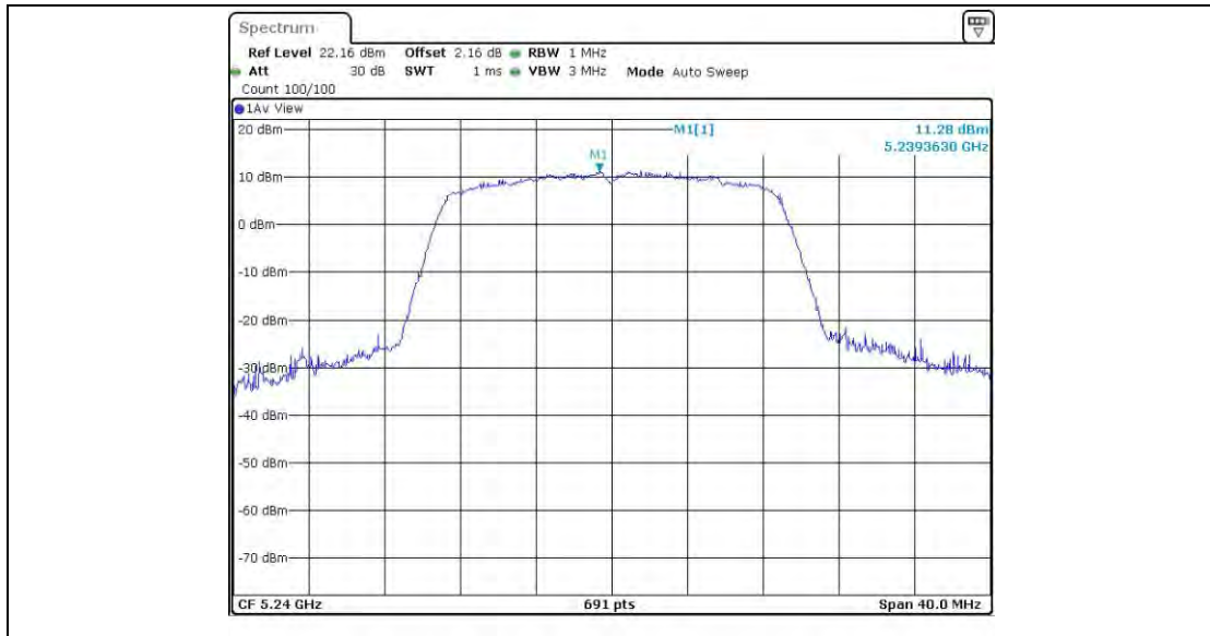
11AC20SISO_Ant4_5240
