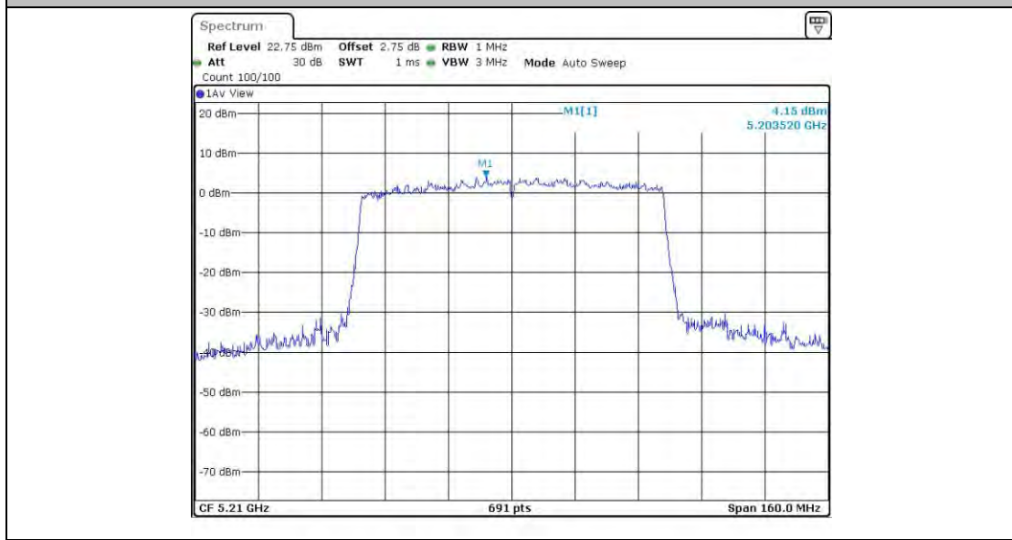
11AC80SISO_Ant3_5210
