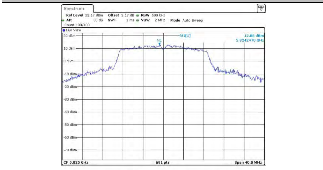
11N20SISO_Ant4_5825
