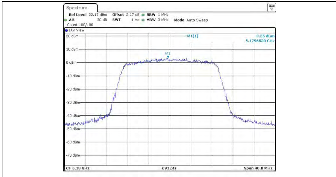
11N20BF_Ant4_5180
