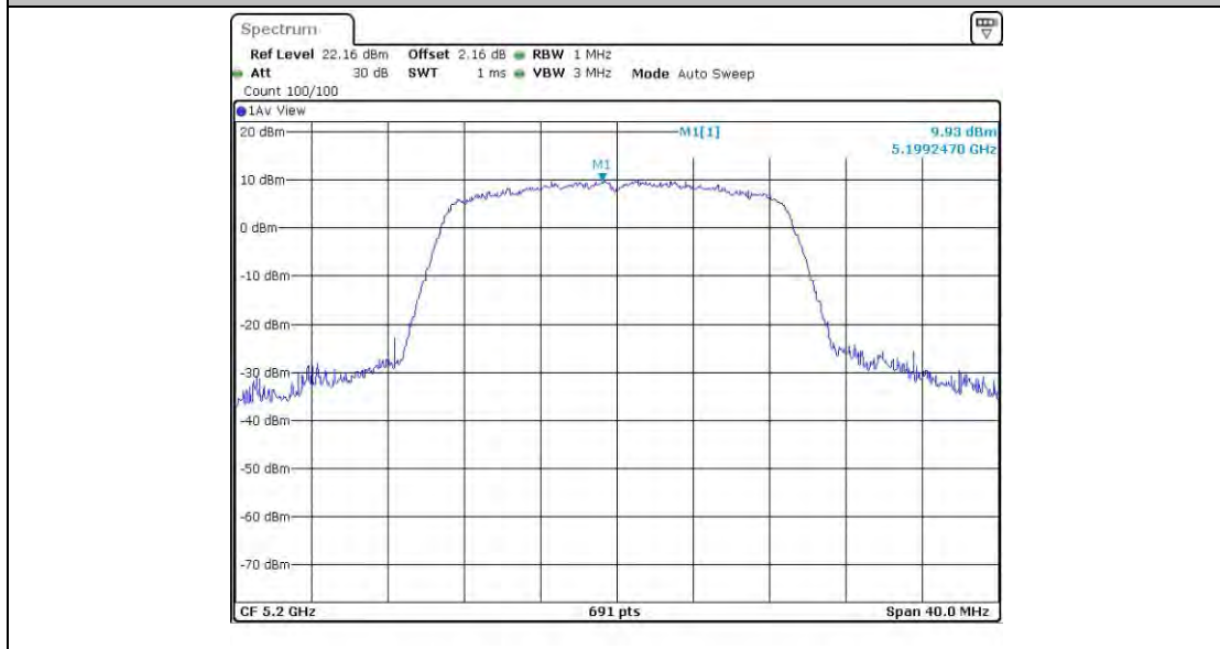
11AC20SISO_Ant4_5200
