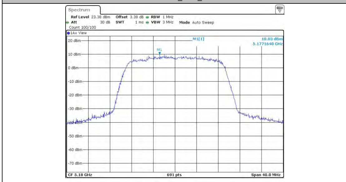
11AC20MIMO_Ant4_5180
