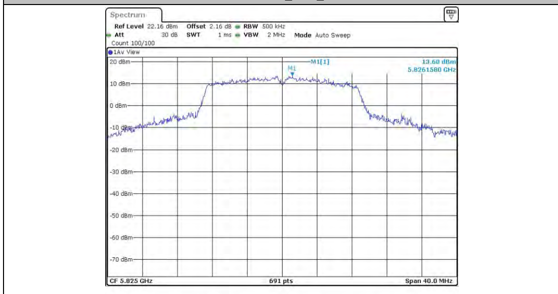
11AC20SISO_Ant3_5825
