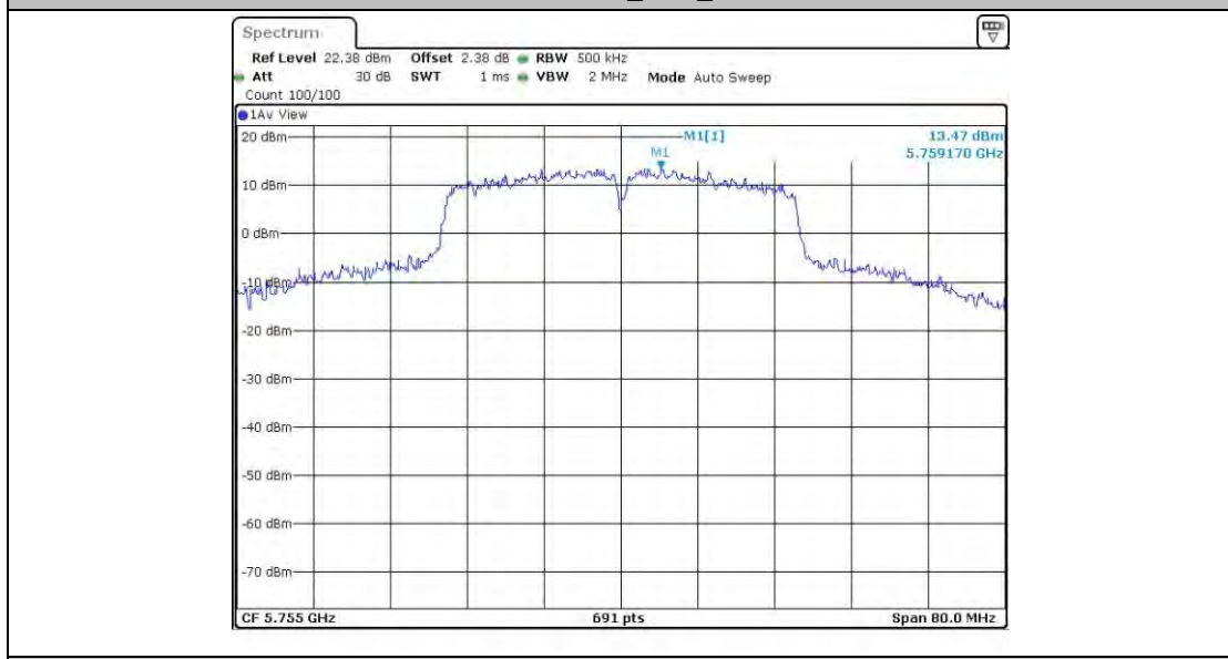
11AC40SISO_Ant3_5755
