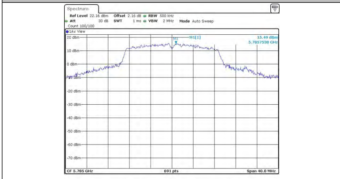
11AC20SISO_Ant3_5785
