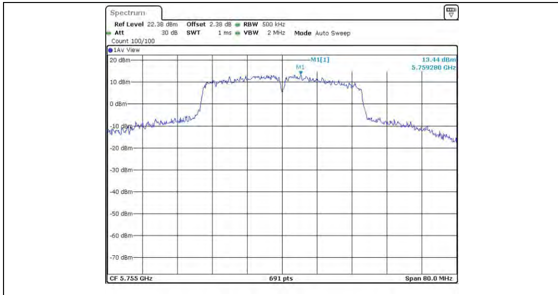
11AC40SISO_Ant4_5755
