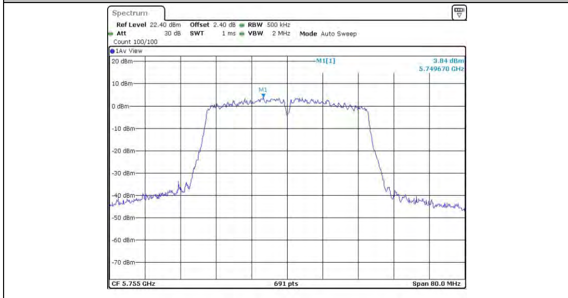
11N40SISO_Ant3_5755
