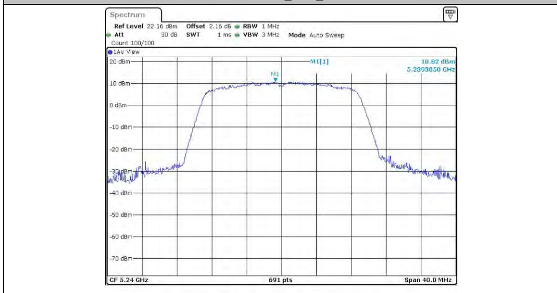
11AC20SISO_Ant3_5240
