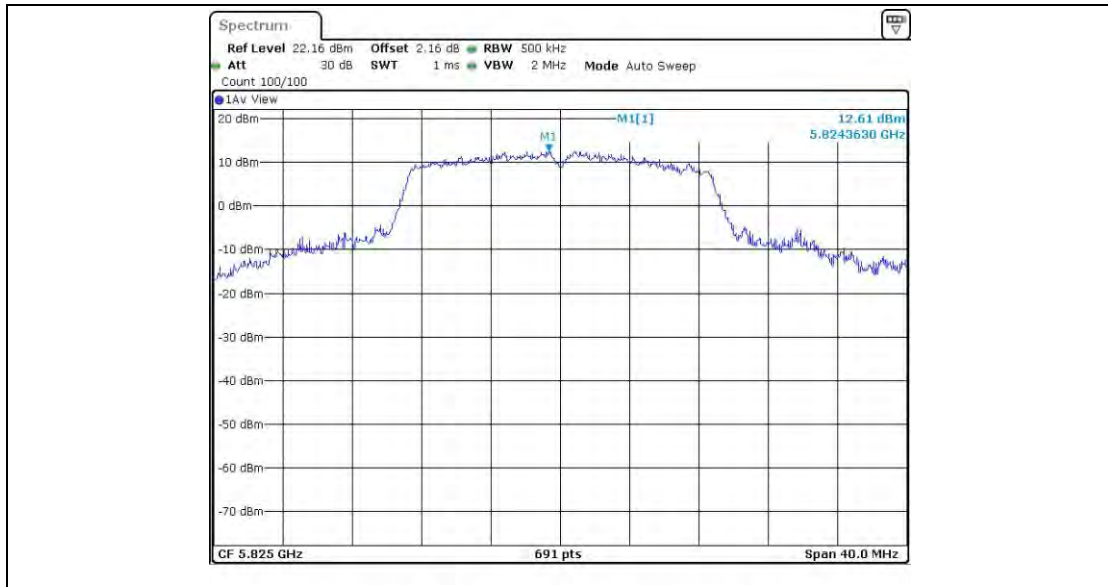
11AC20SISO_Ant4_5825
