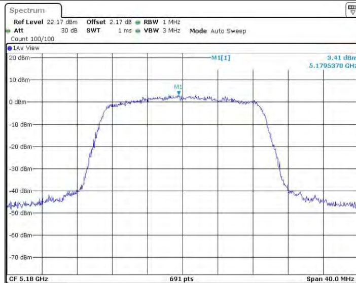
11N20BF_Ant3_5180
