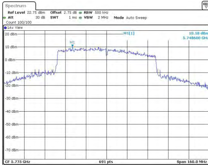
11AC80SISO_Ant4_5775
