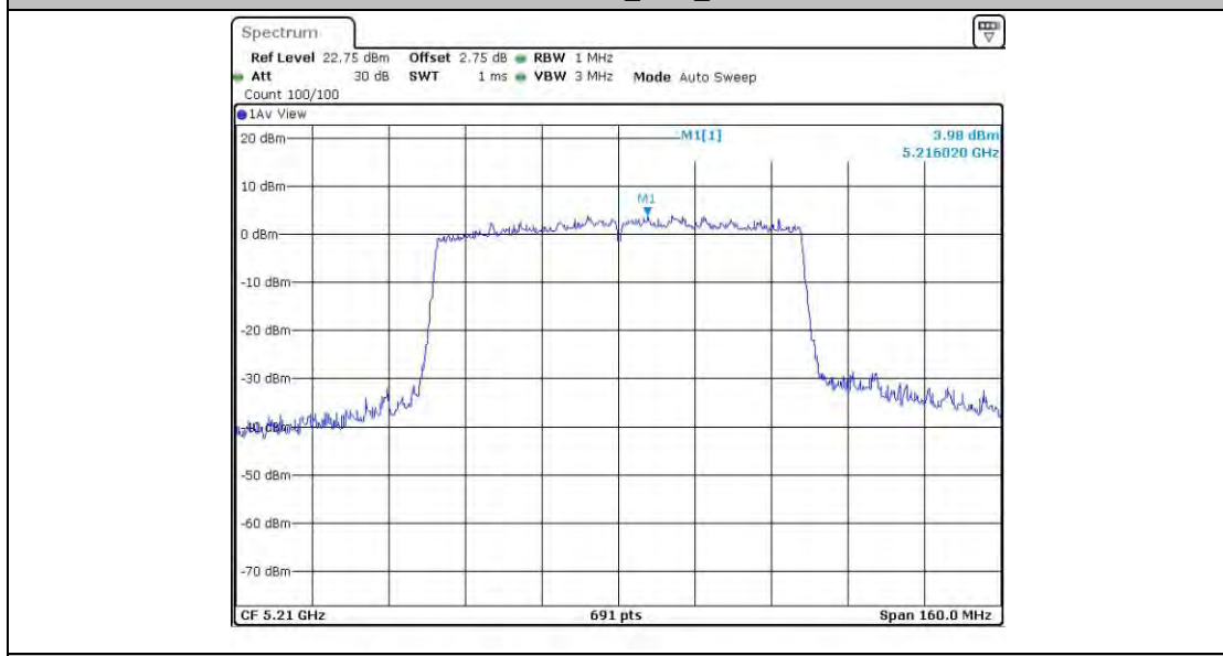
11AC80SISO_Ant4_5210
