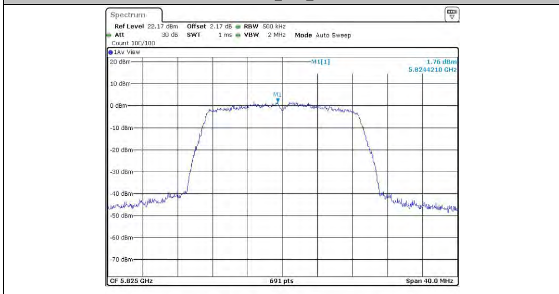
11N20BF_Ant4_5825
