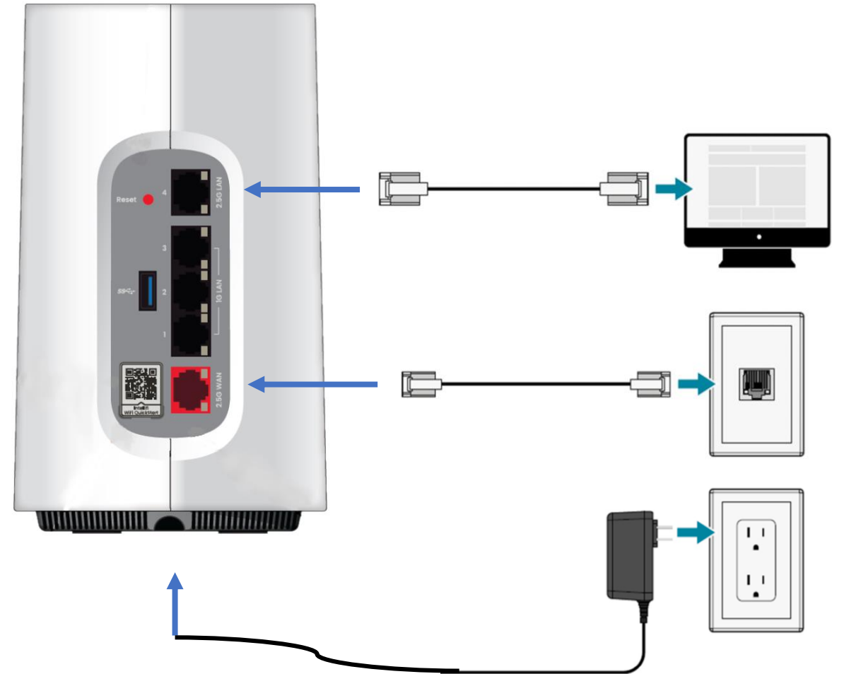
Figure 2. Gateway Installation
