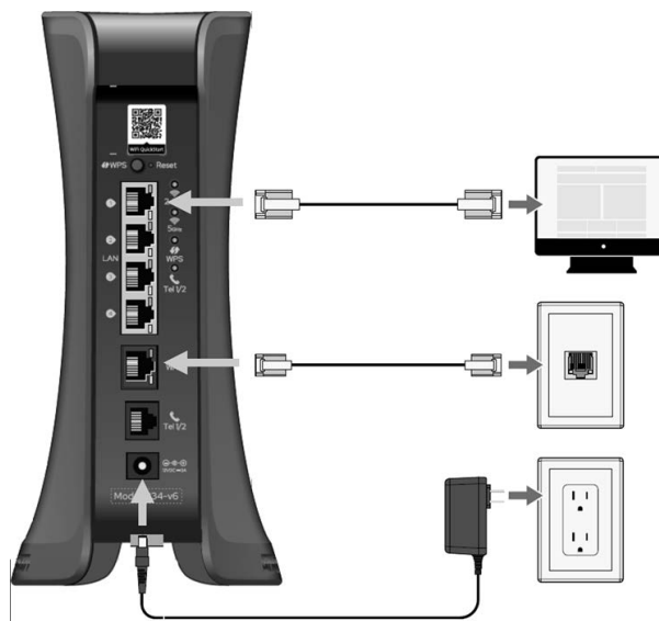
Figure 2. 834-v6 Gateway Installation Options (placeholder)
