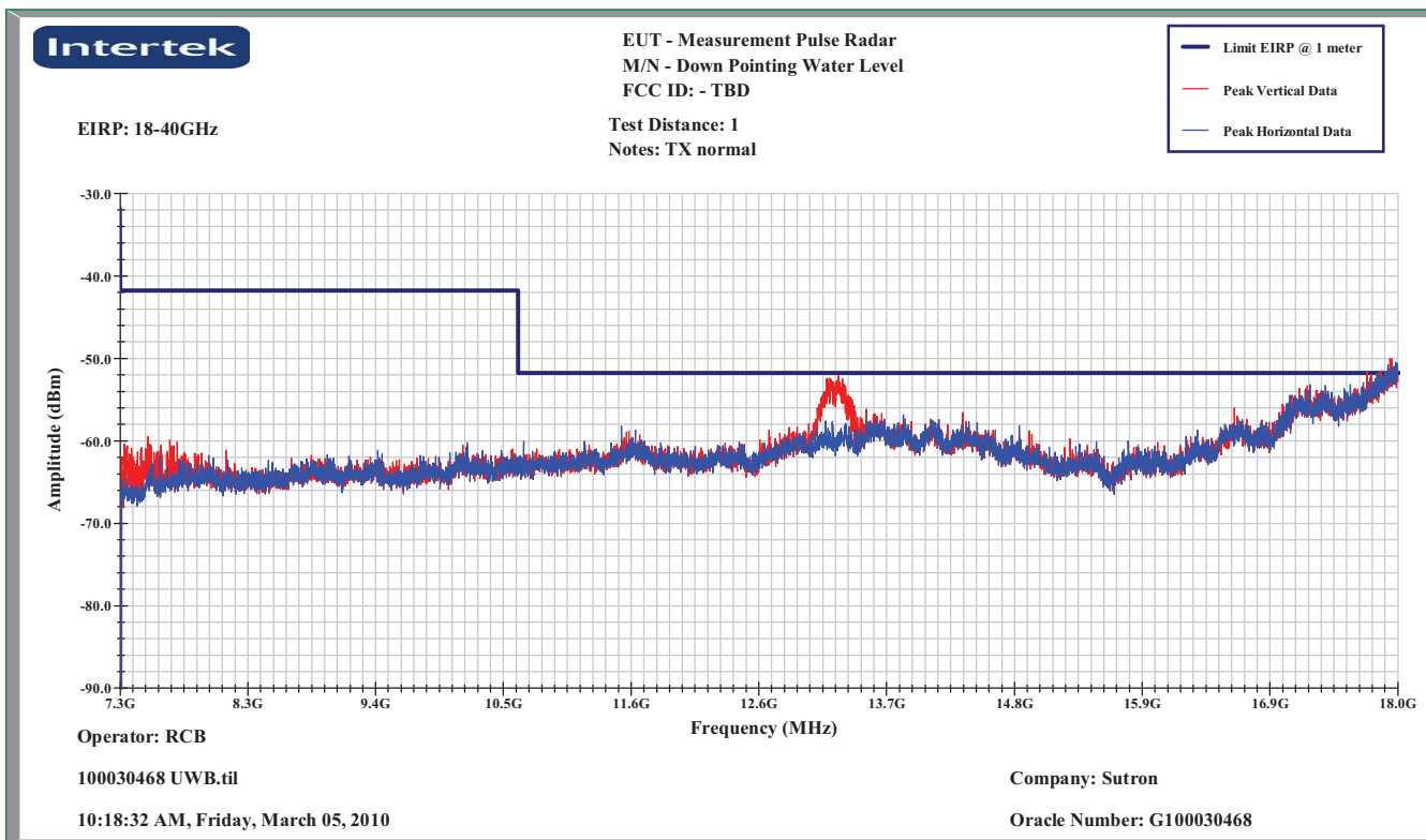
Peak Scan from 7.250 - 18.0GHz
