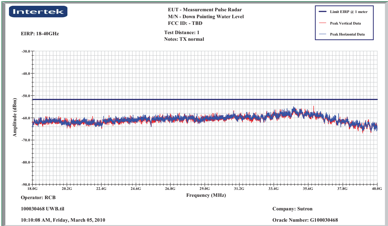
Peak Scan from 18.0 - 40.0GHz
