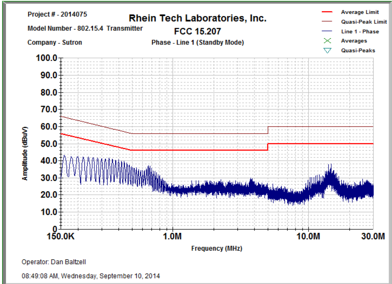
Plot 8-1: Conducted Emissions (Phase Side) (Standby Mode)
