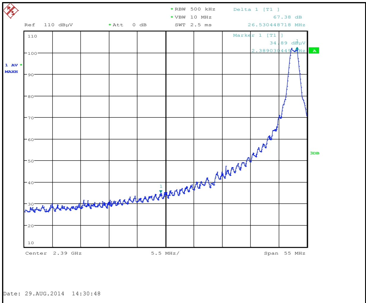
Plot 4-1: Lower Band Edge - 2415 MHz
