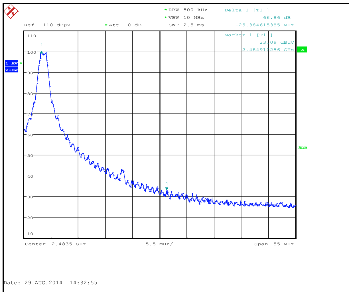
Plot 4-2: Upper Band Edge - 2460 MHz
