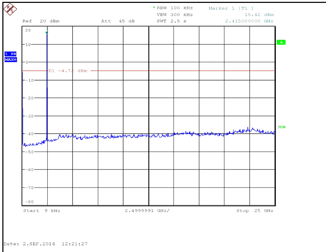
Plot 5-1: Spurious Emissions at Antenna Terminals – 2415 MHz
