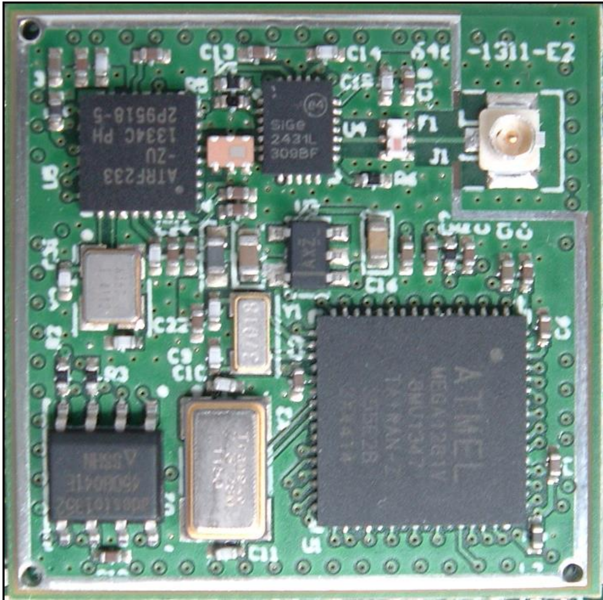
Photograph 12: EUT Top View without Shield
