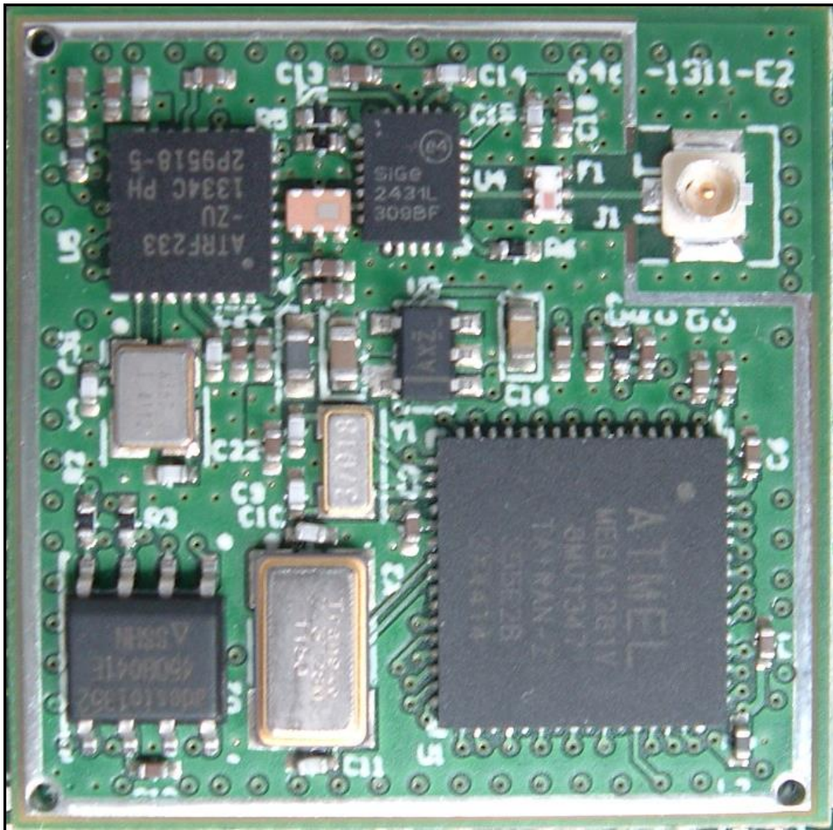
Photograph 8: EUT Top View without Shield
