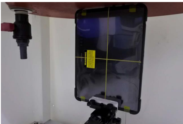
Edge 2 of EUT with Phantom 0 mm Gap
