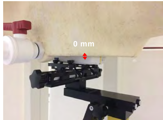
Fig.10 EUT Front side to flat phantom
