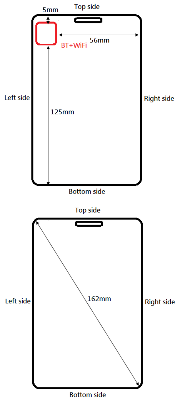
Fig.15 Antenna location and dimensional size
