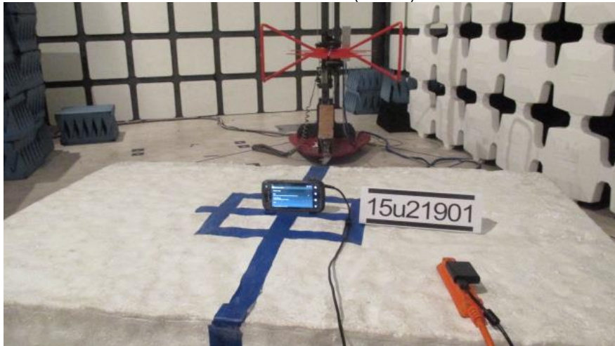
RADIATED EMISSIONS ABOVE 30 MHz (BACK)
