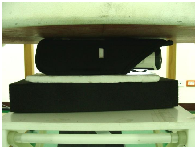
Bottom of the DUT with Holster with Phantom 0 cm Gap
