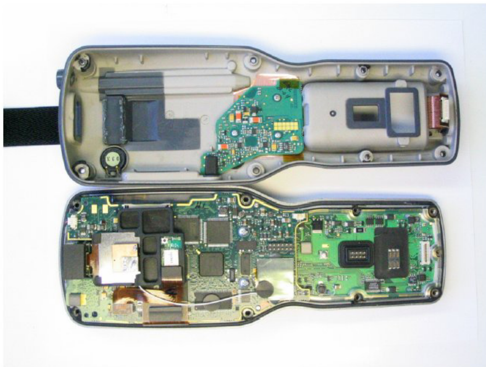
DISASSEMBLED HOUSINGS
