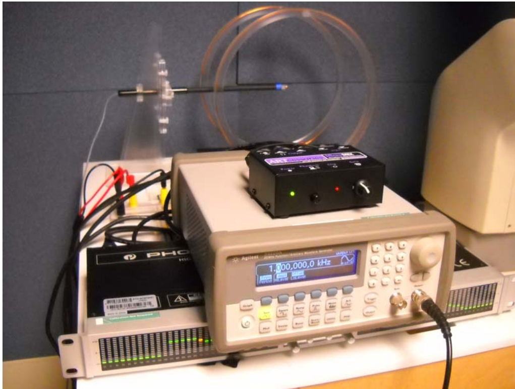
Photo 4: Transverse Probe Calibration
