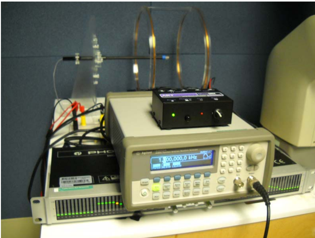
Photo 3: Axial Probe Calibration
