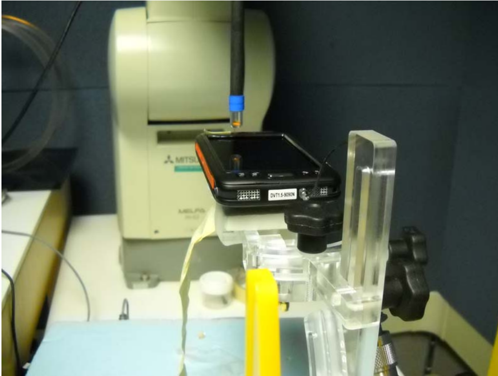
Photo 2: Transverse Probe with Wireless Device
