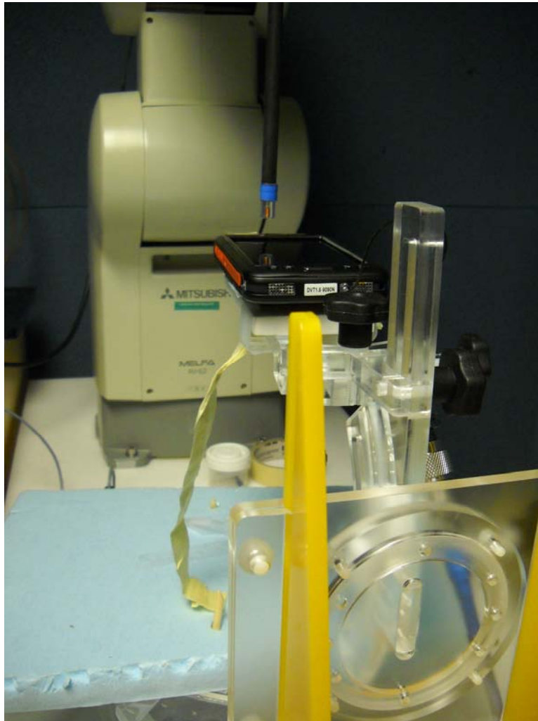
Photo 1: Axial Probe with Wireless Device
