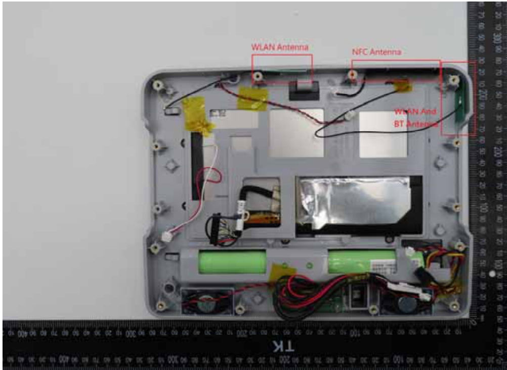
BT+WLAN Antenna
