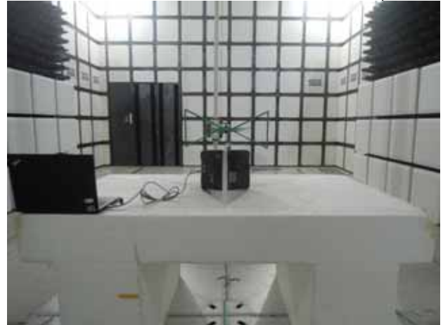
FCC_15_247_BLE_Radiated_External Antenna_Setup
