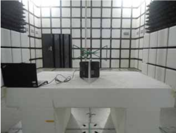
FCC_15_247_BT_Radiated_External Antenna_Setup
