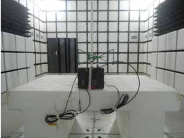
FCC_15_407_Radiated_Internal Antenna_Setup
