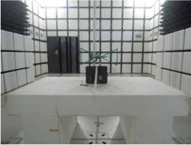
FCC_15_407_Radiated_External Antenna_Setup
