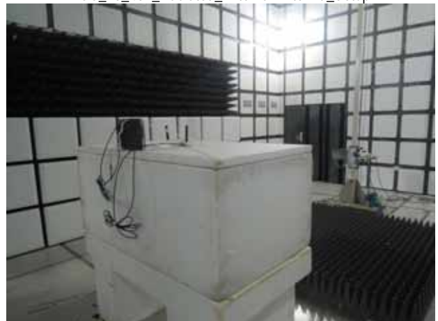
FCC_15_407_Radiated_External Antenna_Setup
