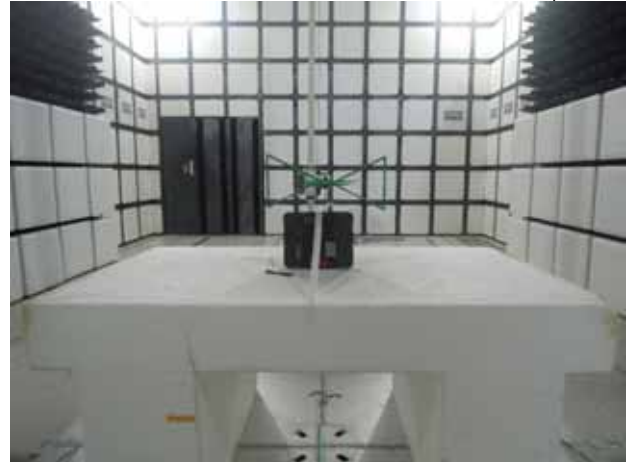
FCC_15_247_WLAN_Radiated_External Antenna_Setup
