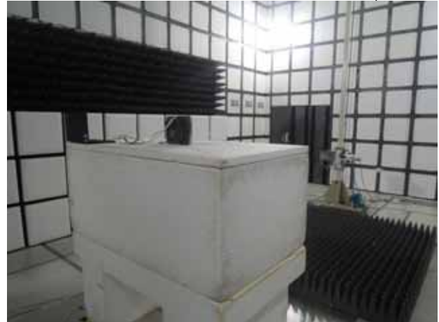
FCC_15_247_BT_Radiated_External Antenna_Setup
