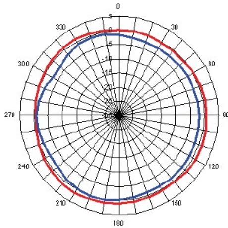
AZIMUTH — 2.5 GHz — 5 GHz
