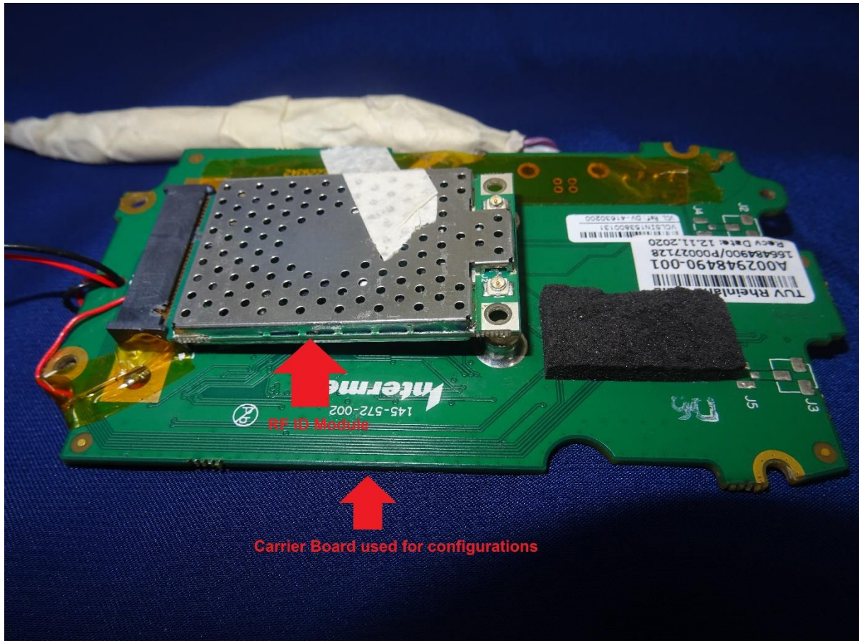
Carrier Board setup used for module configuration
