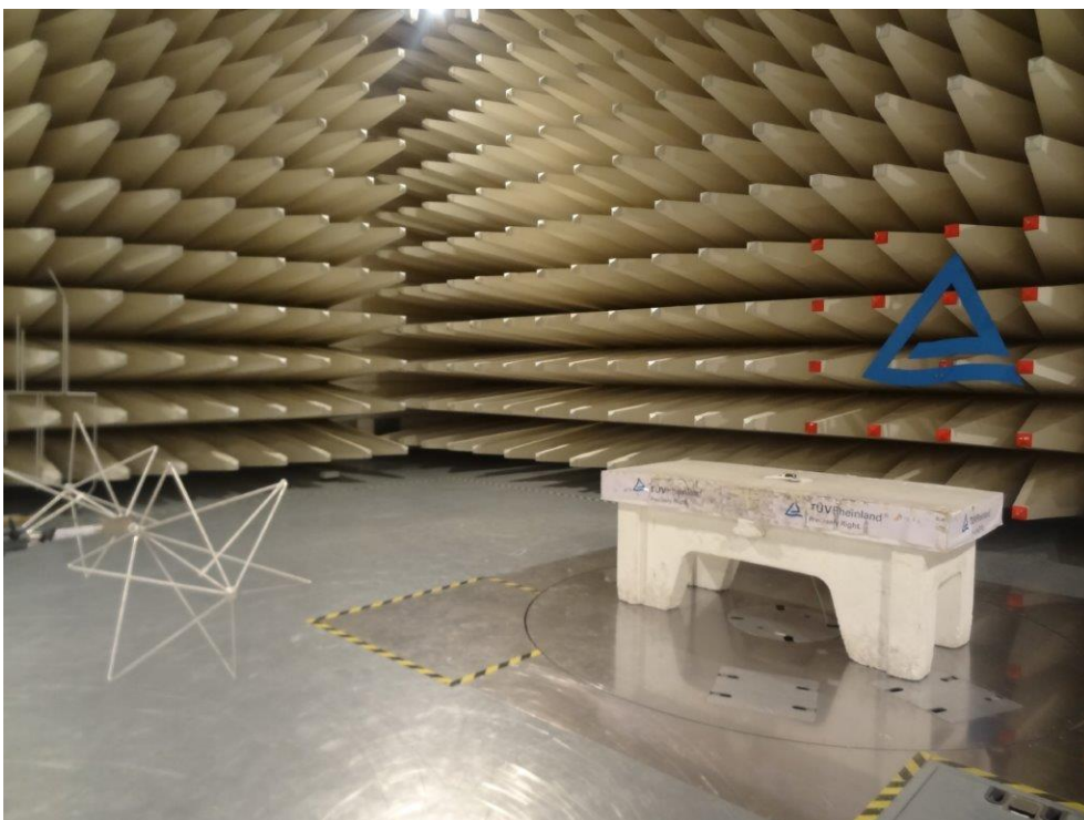
Frequency range:30MHz-200MHz
