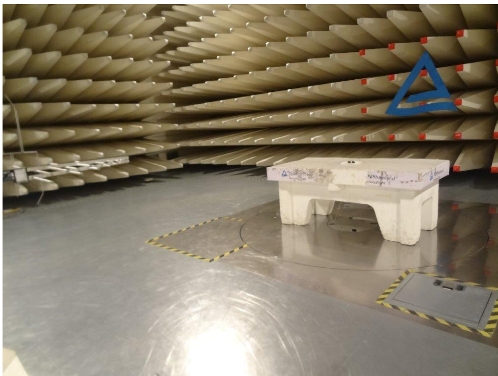
Frequency range:200MHz-1GHz
