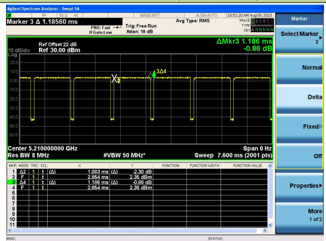
802.11ac-VHT80 (T = 1.083ms)
