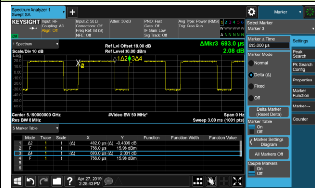
802.11ac-VHT40 (T = 492.0μs)
