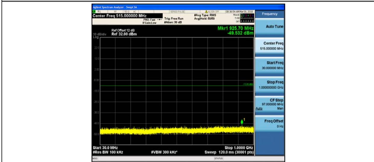
Band2_1.4MHz_QPSK_18900_1RB#0
