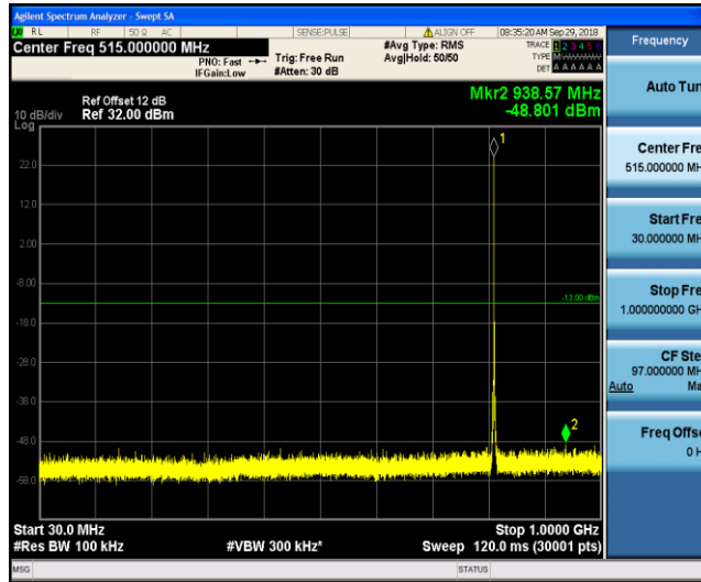
Band26_1.4MHz_QPSK_26697_1RB#0
