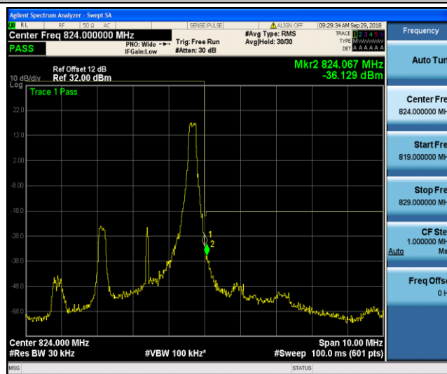
Band26_3MHz_16QAM_26775_1RB#14
