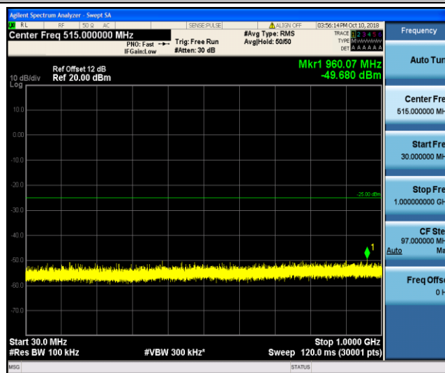
Band41_10MHz_16QAM_40740_1RB#0
