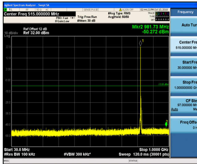
Band26_5MHz_16QAM_20425_1RB#0
