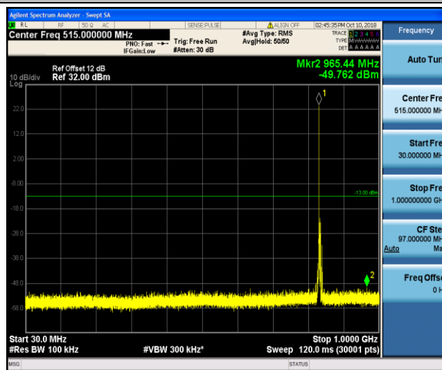
Band26_5MHz_16QAM_20525_1RB#0
