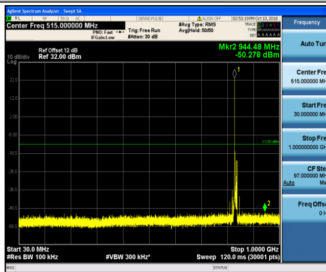
Band26_10MHz_QPSK_20525_1RB#0
