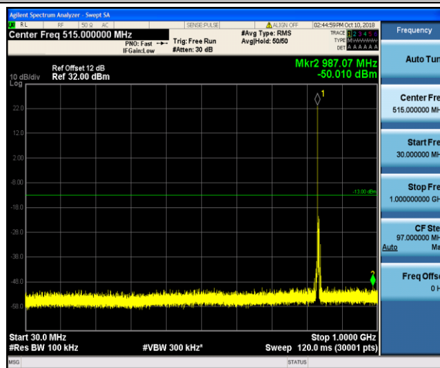
Band26_5MHz_QPSK_20525_1RB#0
