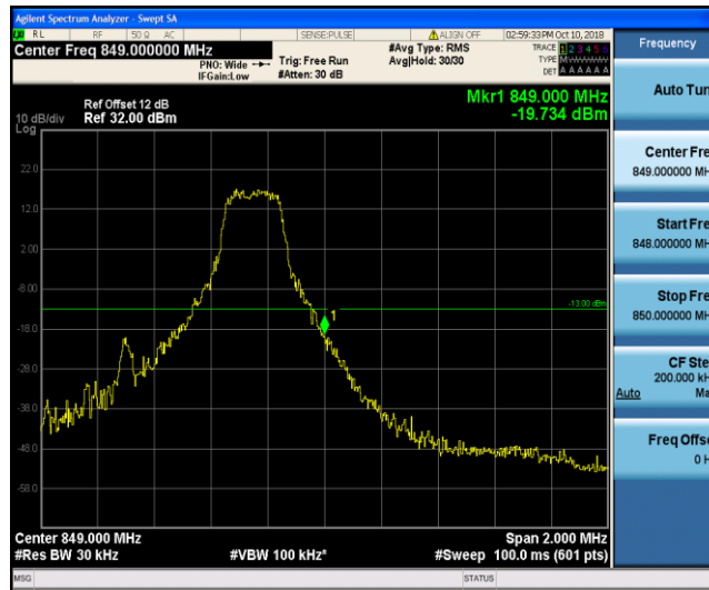
Band26_1.4MHz_16QAM_20643_1RB#5
