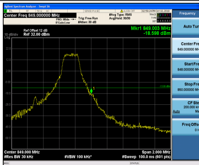
Band26_1.4MHz_QPSK_20643_1RB#5
