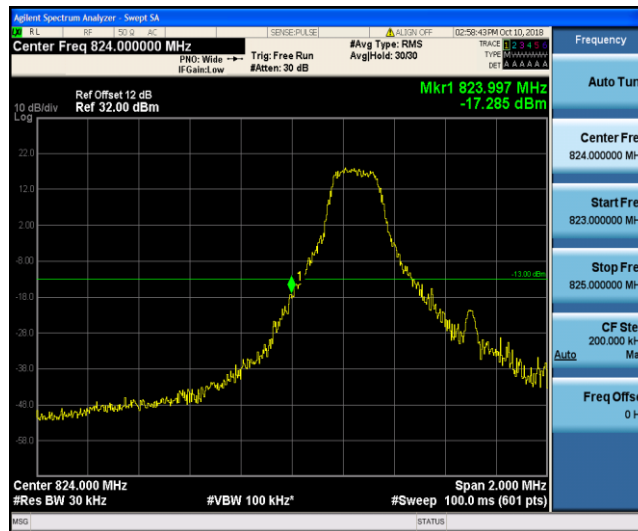
Band26_1.4MHz_QPSK_20407_1RB#0
