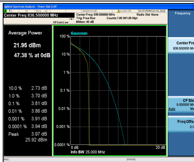
Band26_3MHz_QPSK_20525_1RB#0
