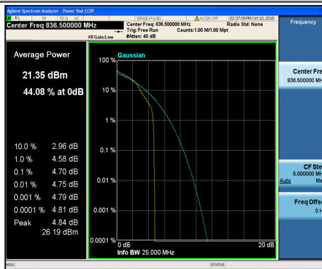
Band26_3MHz_16QAM_20525_1RB#0
