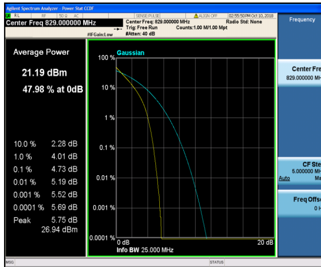
Band26_10MHz_QPSK_20450_50RB#0
