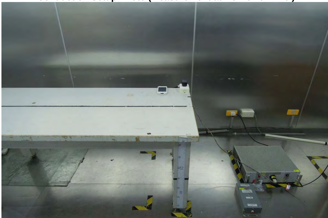
Conduction Setup Photo (Measurement at AC Power Line )
