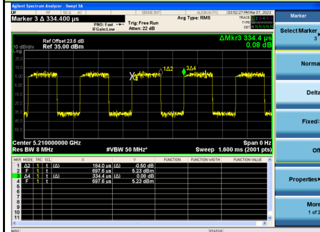
802.11ax-HE80 (T = 184.0us)
