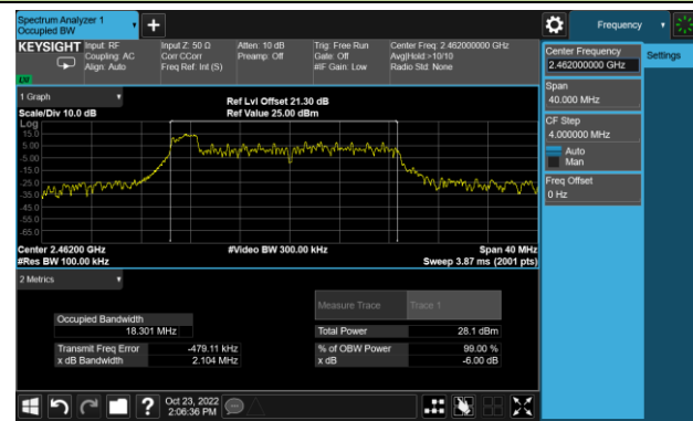
Channel 11 (2462MHz)
