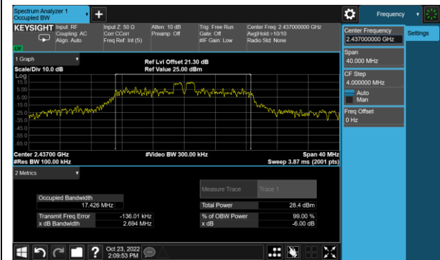
Channel 06 (2437MHz)
