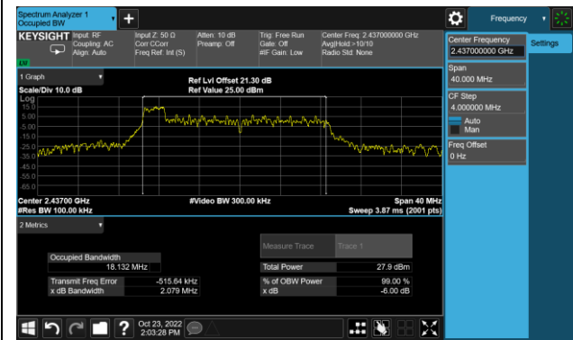
Channel 06 (2437MHz)
