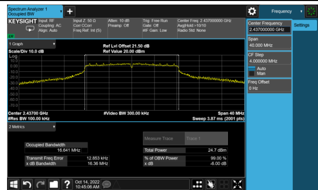
Channel 06 (2437MHz)
