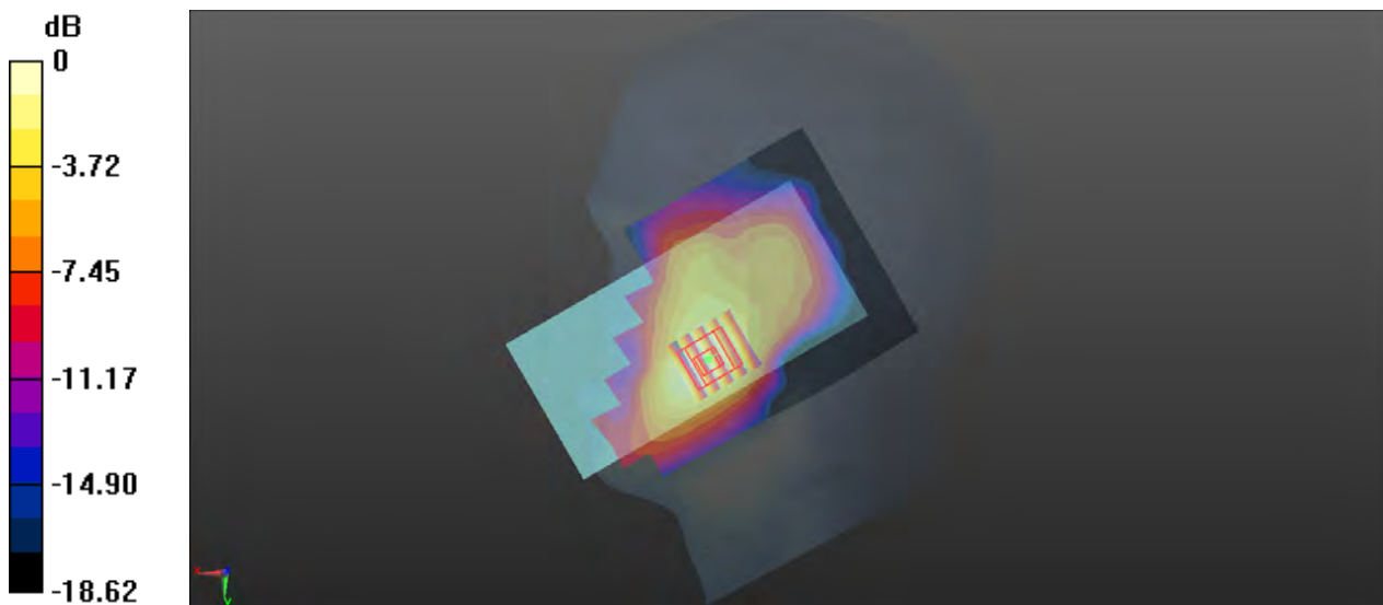
0 dB = 0.171 W/kg
