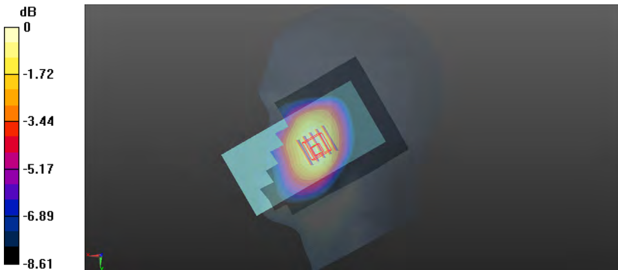
0 dB = 0.474 W/kg
