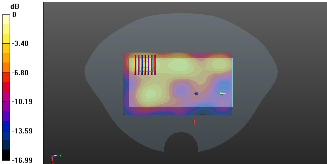
0 dB = 0.0694 W/kg
