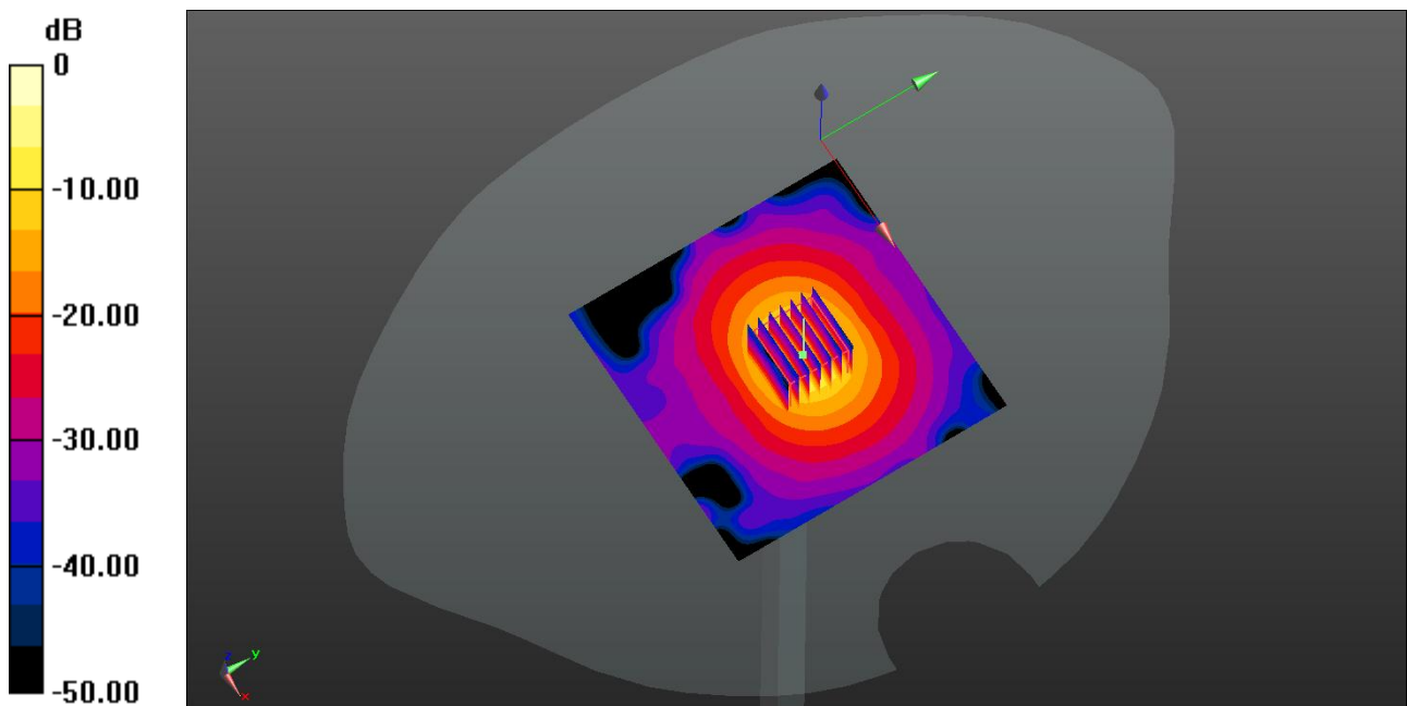
0 dB = 15.6 W/kg
