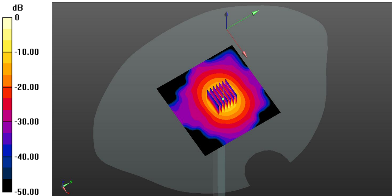
0 dB = 15.2 W/kg
