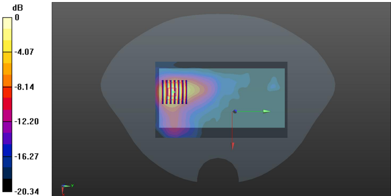
0 dB = 0.183 W/kg
