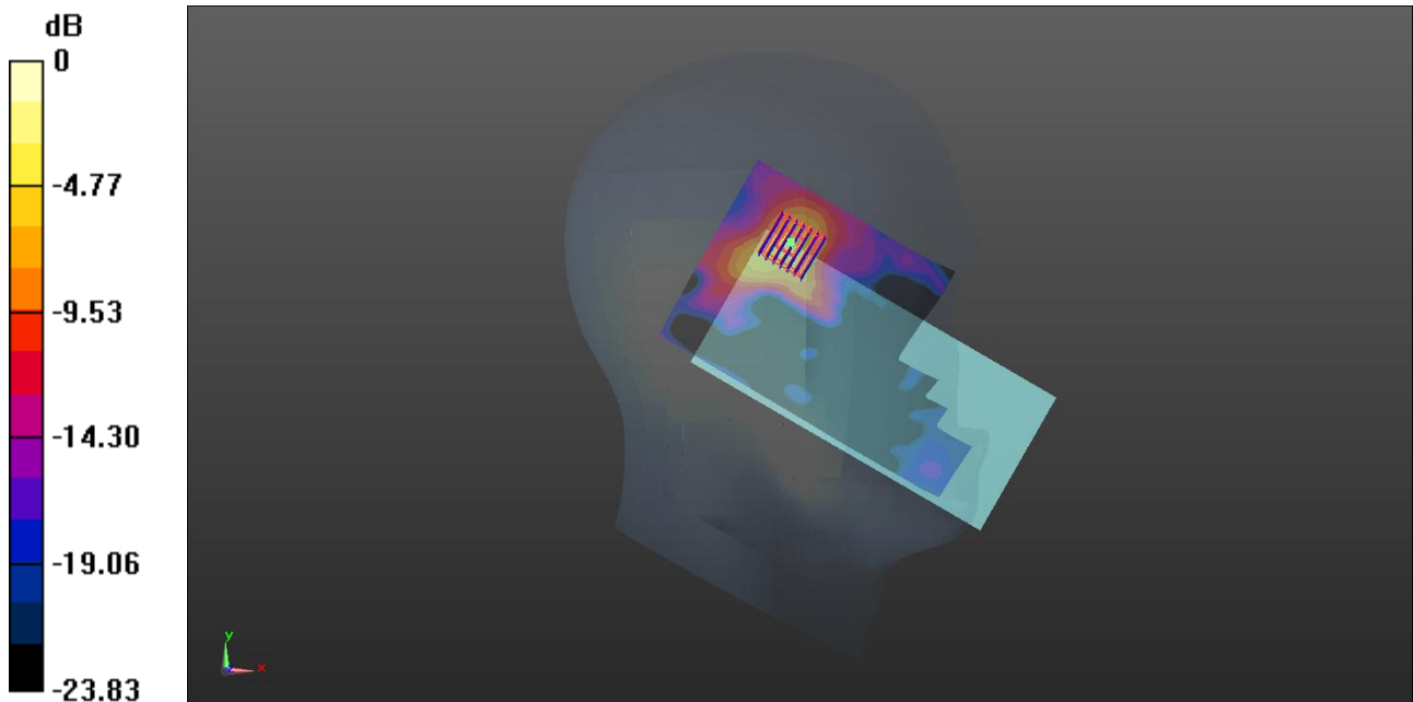
0 dB = 0.451 W/kg
