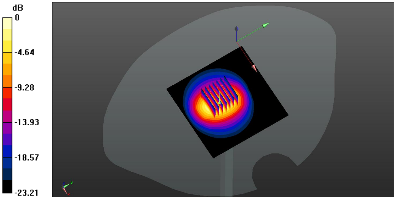
0 dB = 6.28 W/kg
