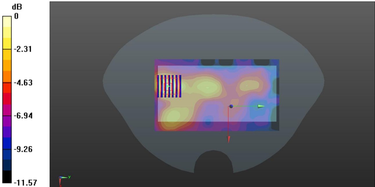
0 dB = 0.0145 W/kg
