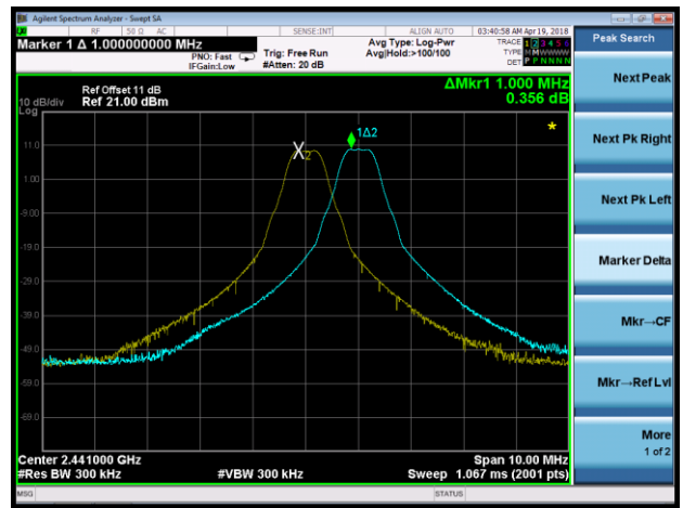
Channel 39 (2441MHz)
