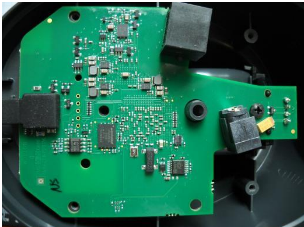
Fig.6: PCB View-1
