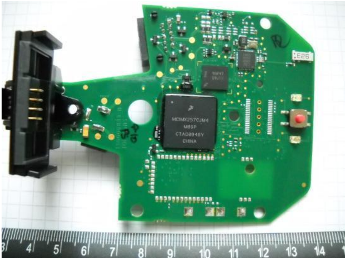
Fig.7: PCB View-2
