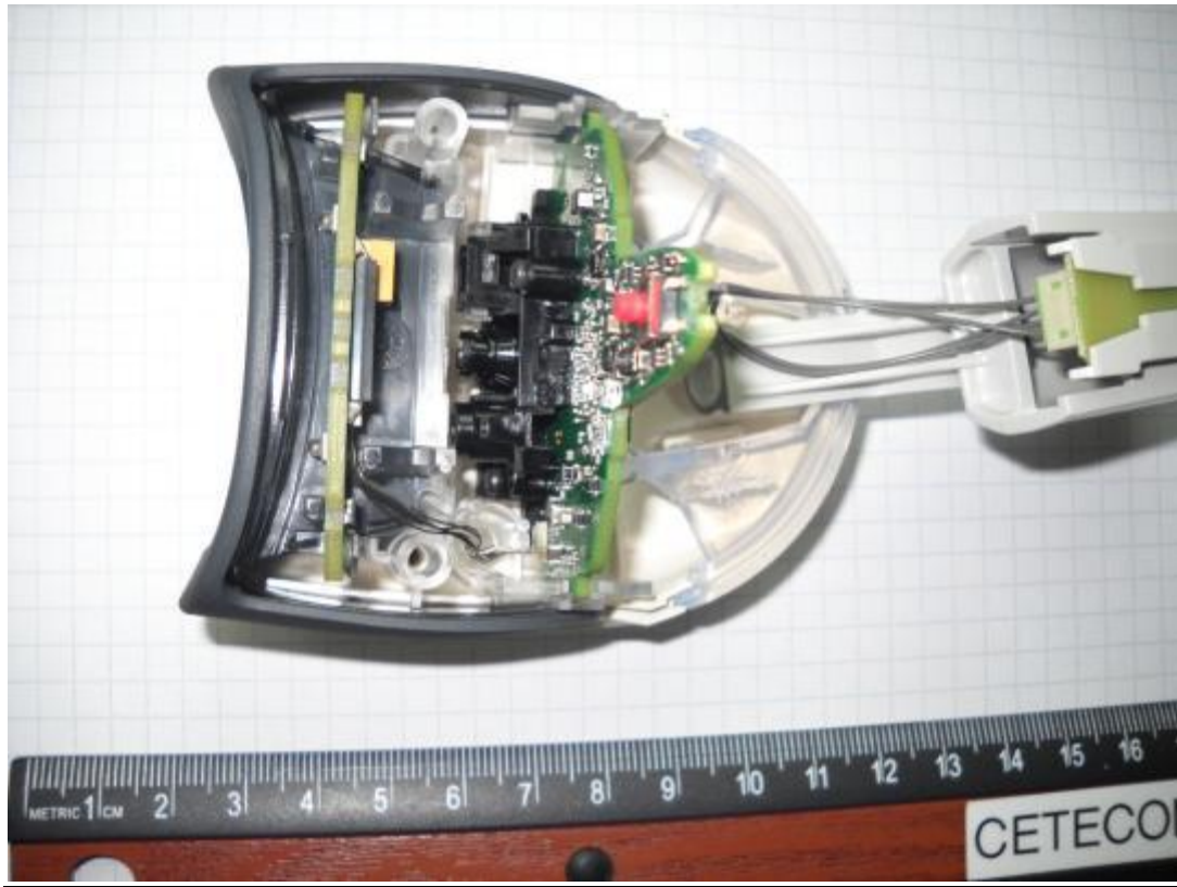
Fig.3: Internal view-1
