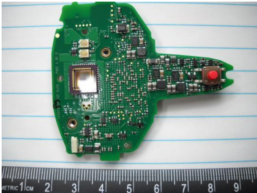
Fig.8: PCB View-2
