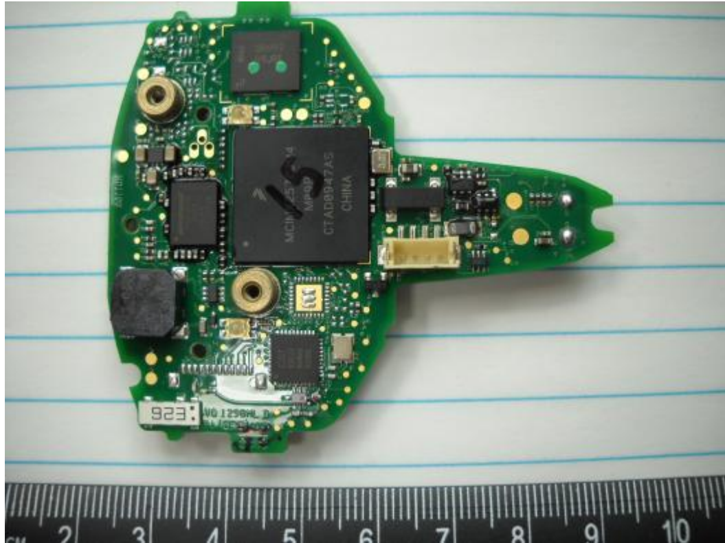
Fig.9: PCB View-3
