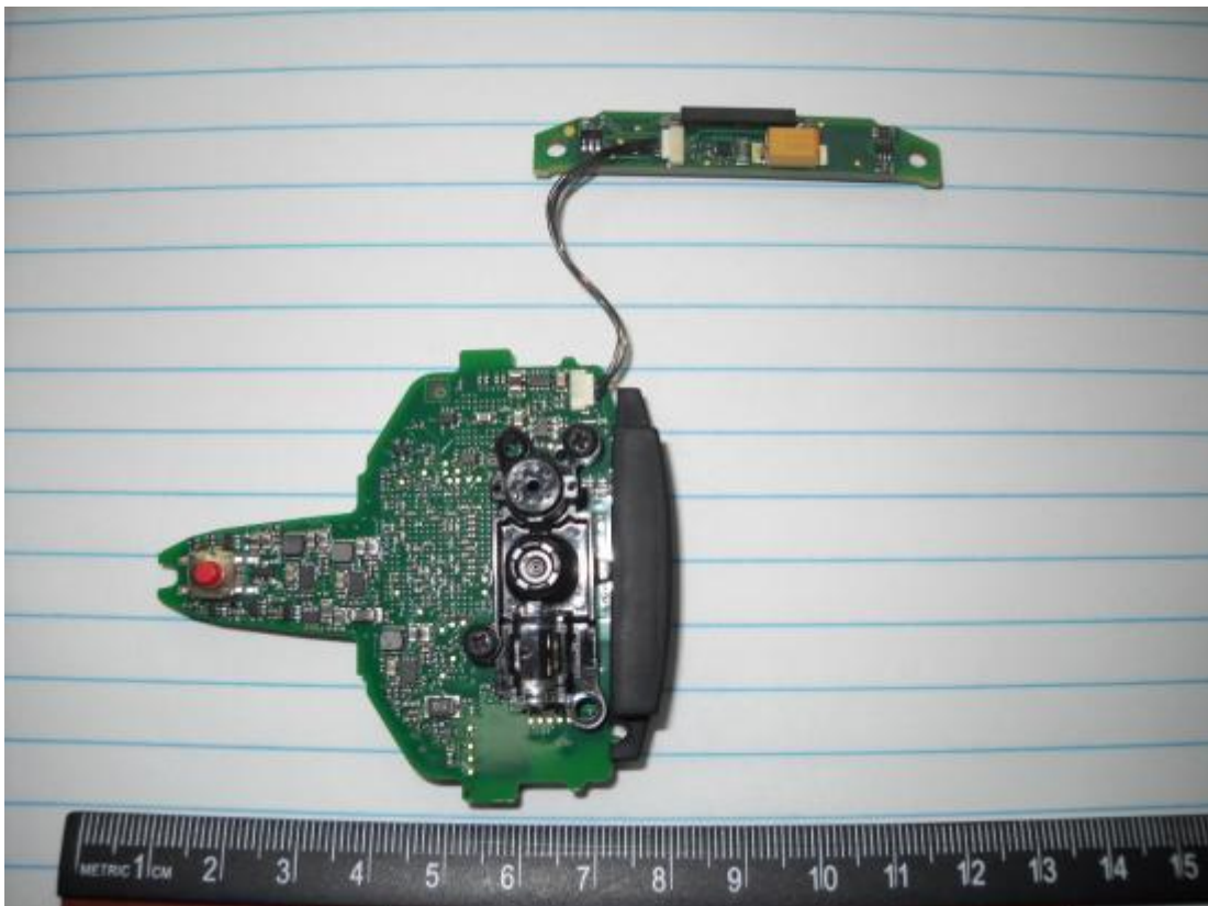
Fig.6: Internal View-4
