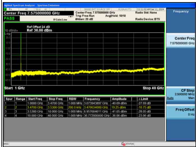
CSE_MIMO(ANT5)_n77(K)_30KHz_64QAM_50M CH635000_1RB@1_
