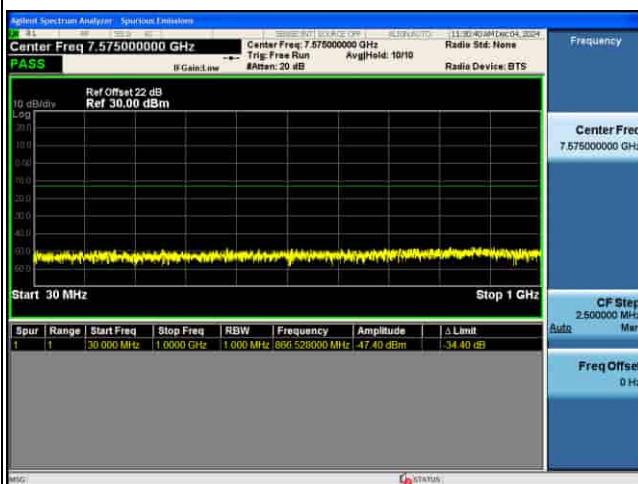
CSE_5G_n77(N)_30KHz_256QAM_30M CH664332_1RB@1_
