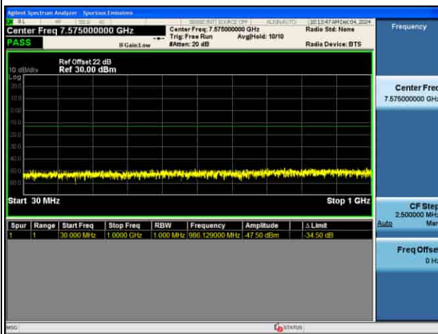
CSE_5G_n77(N)_30KHz_256QAM_15M CH656000_1RB@1_
