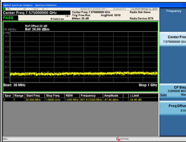
CSE_MIMO(ANT5)_n77(K)_30KHz_QPSK_50M CH633334_1RB@1_
