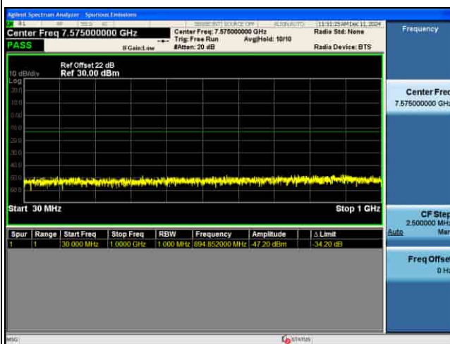
CSE_MIMO(ANT5)_n77(K)_30KHz_QPSK_40M CH635332_1RB@1_
