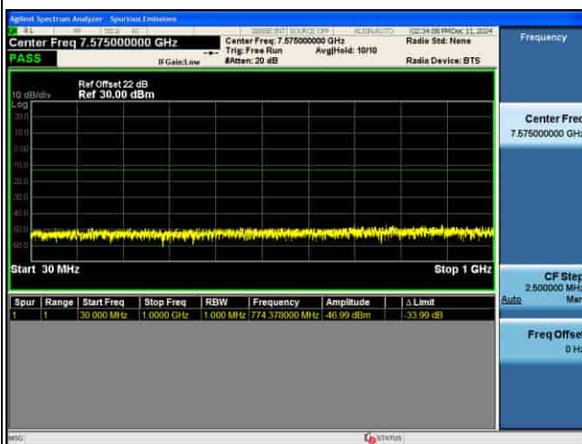
CSE_MIMO(ANT5)_n77(K)_30KHz_16QAM_30M CH633334_1RB@1_
