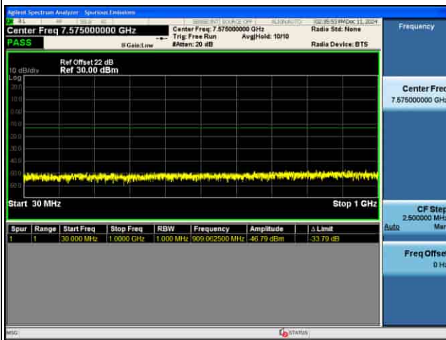
CSE_MIMO(ANT5)_n77(K)_30KHz_QPSK_30M CH633334_1RB@1_
