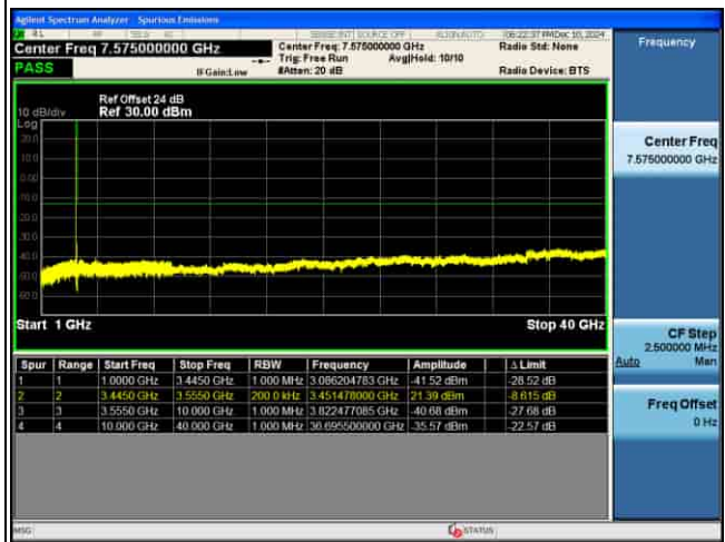
CSE_MIMO(ANT5)_n77(K)_30KHz_16QAM_10M CH630334_1RB@1_
