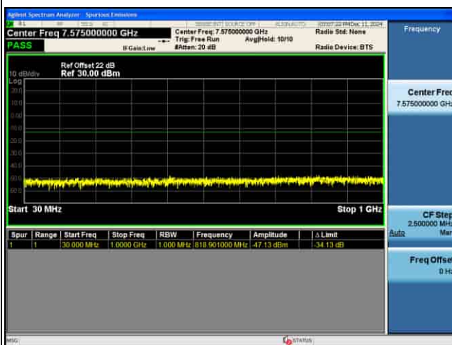
CSE_MIMO(ANT5)_n77(K)_30KHz_64QAM_20M CH630668_1RB@1_
