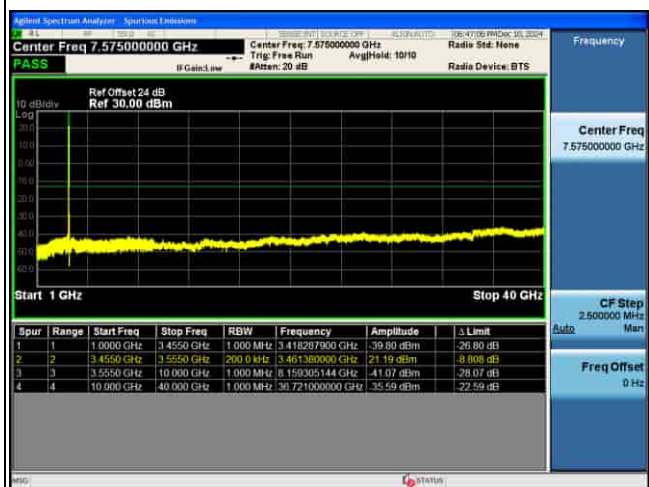
CSE_MIMO(ANT5)_n77(K)_30KHz_QPSK_90M CH633666_1RB@1_
