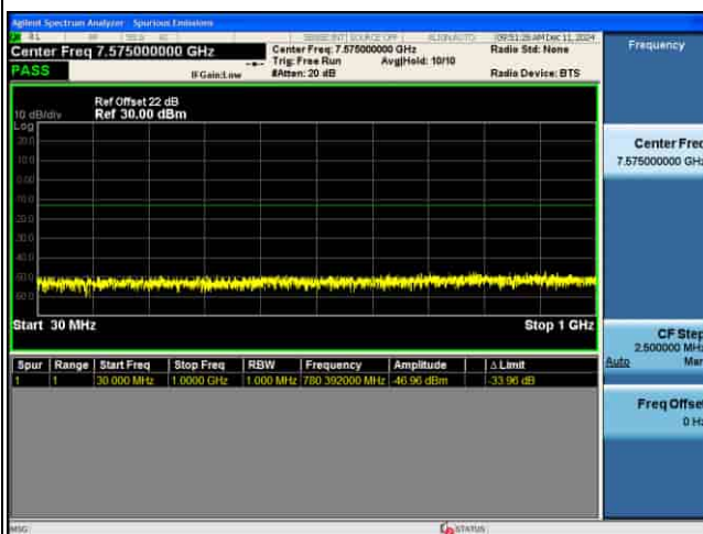
CSE_MIMO(ANT5)_n77(K)_30KHz_QPSK_80M CH634000_1RB@1_
