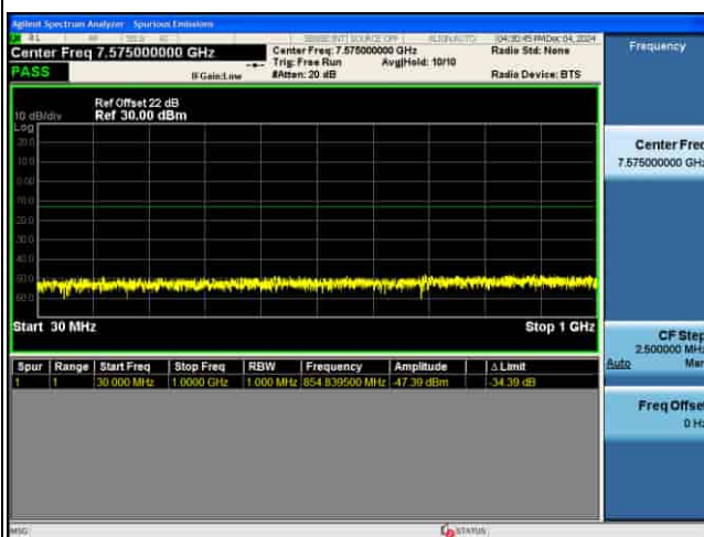
CSE_5G_n77(N)_30KHz_256QAM_90M CH662332_1RB@1_
