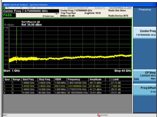
CSE_MIMO(ANT5)_n77(K)_30KHz_16QAM_30M CH633334_1RB@1_
