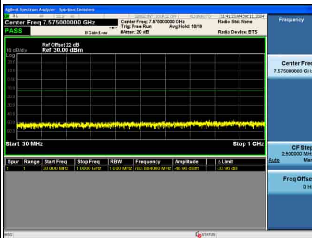
CSE_MIMO(ANT5)_n77(K)_30KHz_64QAM_50M CH631668_1RB@1_
