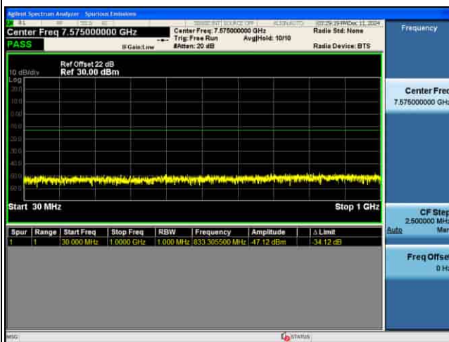
CSE_MIMO(ANT5)_n77(K)_30KHz_64QAM_15M CH630500_1RB@1_
