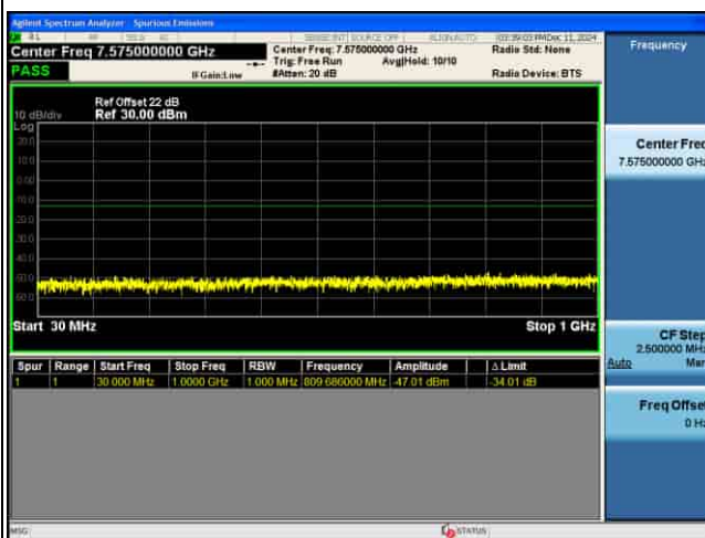
CSE_MIMO(ANT5)_n77(K)_30KHz_16QAM_10M CH633334_1RB@1
