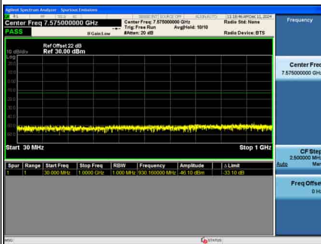
CSE_MIMO(ANT5)_n77(K)_30KHz_16QAM_50M CH633334_1RB@1_
