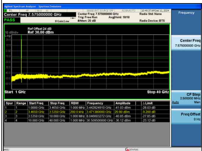
CSE_MIMO(ANT5)_n77(K)_30KHz_16QAM_60M CH633334_1RB@1_
