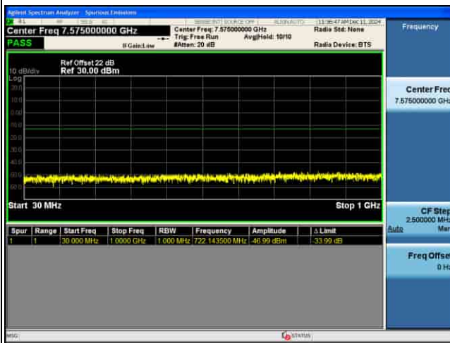
CSE_MIMO(ANT5)_n77(K)_30KHz_16QAM_50M CH631668_1RB@1_
