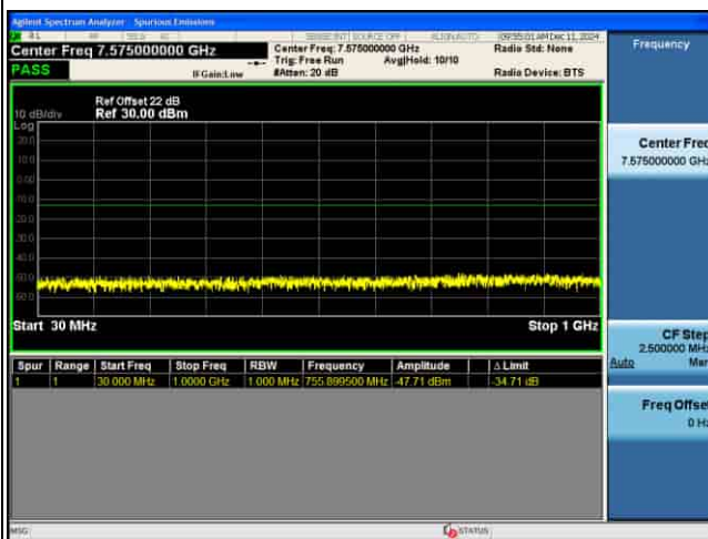
CSE_MIMO(ANT5)_n77(K)_30KHz_QPSK_80M CH634000_1RB@1_
