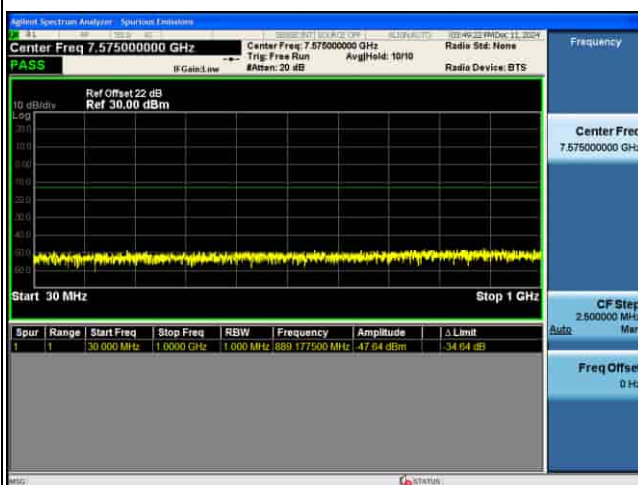
CSE_MIMO(ANT5)_n77(K)_30KHz_QPSK_15M CH636166_1RB@1_
