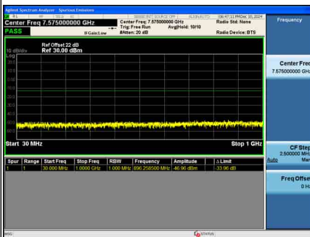
CSE_MIMO(ANT5)_n77(K)_30KHz_QPSK_90M CH633666_1RB@1_
