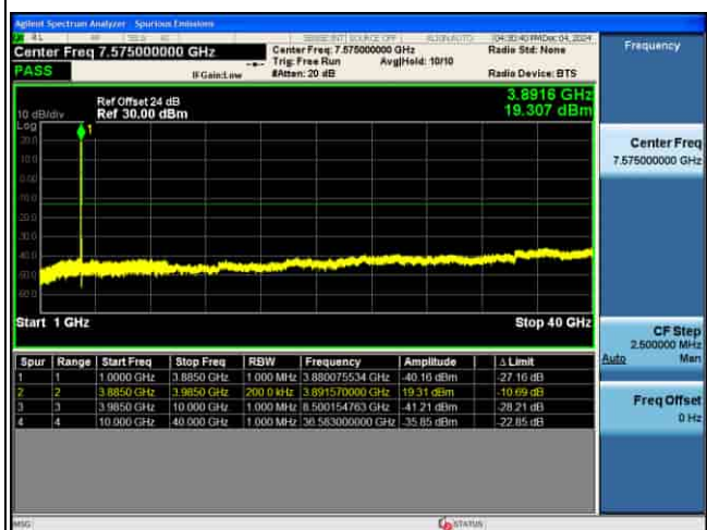
CSE_5G_n77(N)_30KHz_256QAM_90M CH662332_1RB@1_
