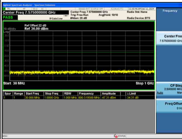
CSE_MIMO(ANT5)_n77(K)_30KHz_QPSK_40M CH633334_1RB@1_
