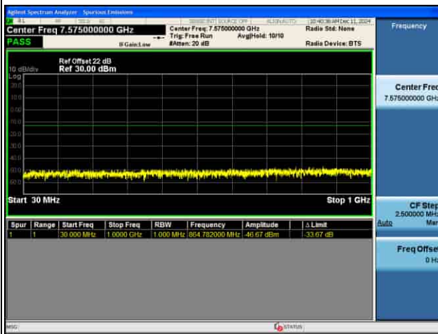
CSE_MIMO(ANT5)_n77(K)_30KHz_QPSK_60M CH633334_1RB@1_
