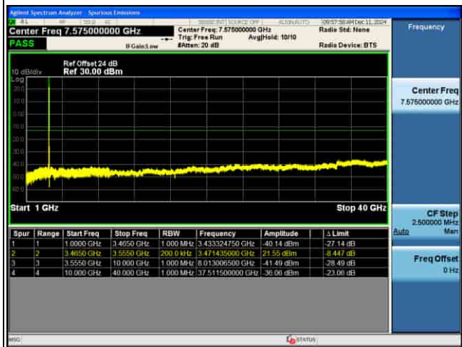
CSE_MIMO(ANT5)_n77(K)_30KHz_16QAM_90M CH633000_1RB@1_
