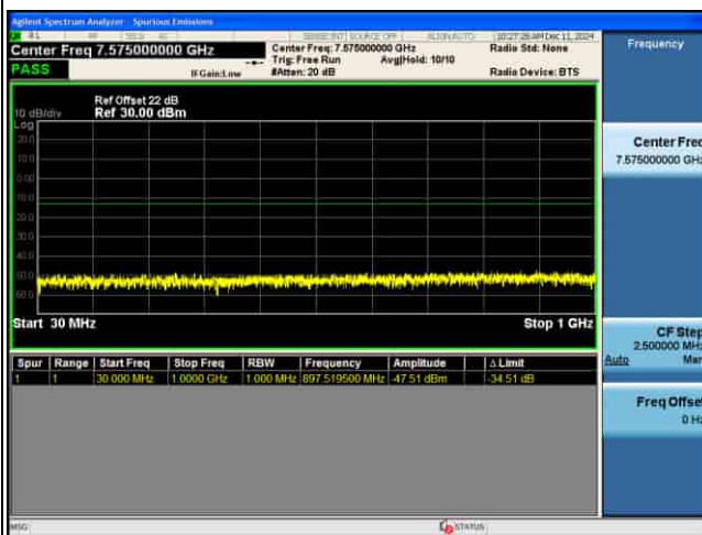
CSE_MIMO(ANT5)_n77(K)_30KHz_16QAM_70M CH633334_1RB@1_
