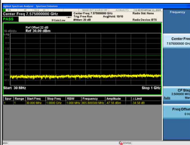
CSE_MIMO(ANT5)_n77(K)_30KHz_64QAM_40M CH631334_1RB@1_
