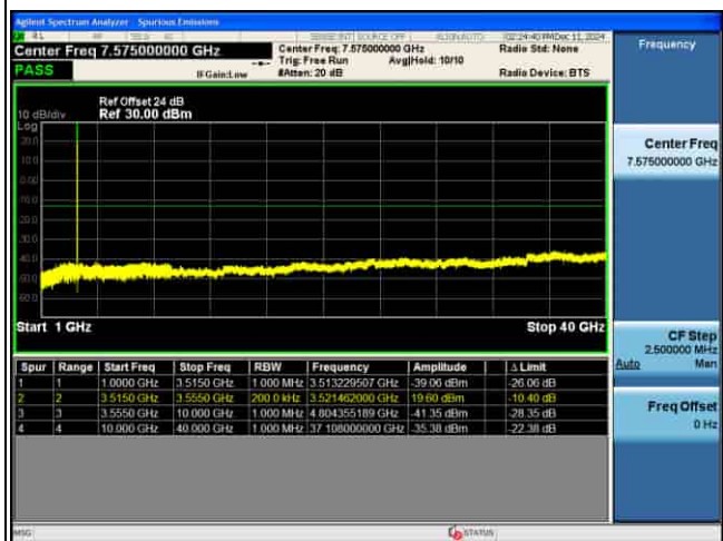
CSE_MIMO(ANT5)_n77(K)_30KHz_64QAM_40M CH631334_1RB@1_
