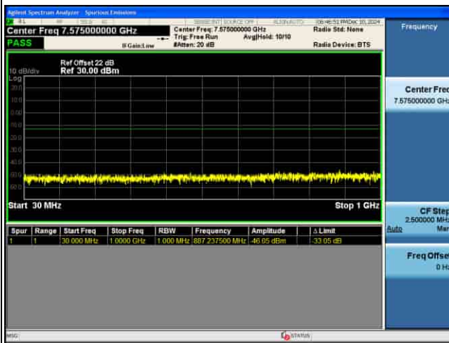
CSE_MIMO(ANT5)_n77(K)_30KHz_QPSK_90M CH633334_1RB@1_
