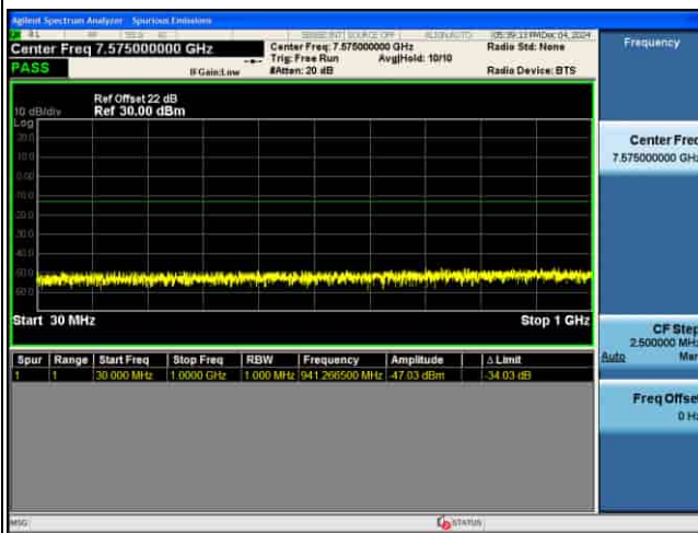
CSE_5G_n77(N)_30KHz_256QAM_100M CH656000_1RB@1
