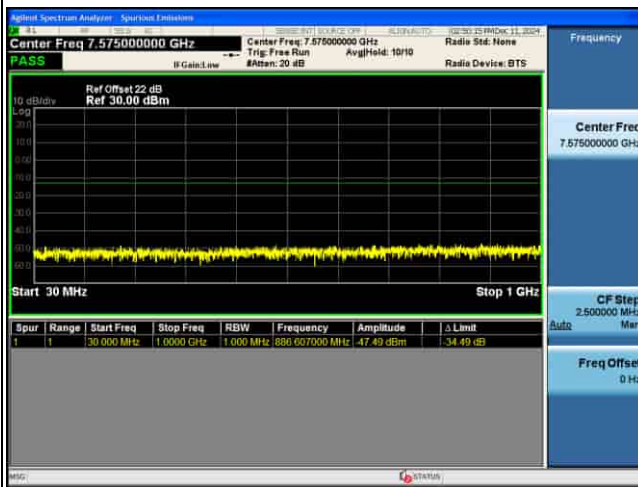
CSE_MIMO(ANT5)_n77(K)_30KHz_QPSK_20M CH633334_1RB@1_
