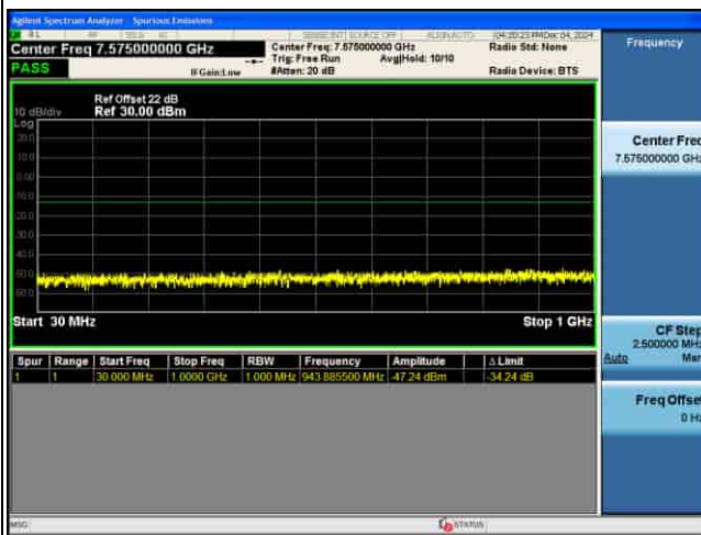
CSE_5G_n77(N)_30KHz_256QAM_80M CH656000_1RB@1_
