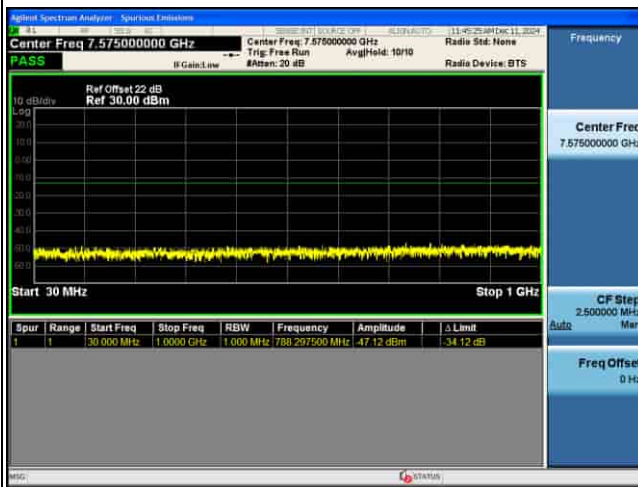
CSE_MIMO(ANT5)_n77(K)_30KHz_64QAM_40M CH635332_1RB@1_
