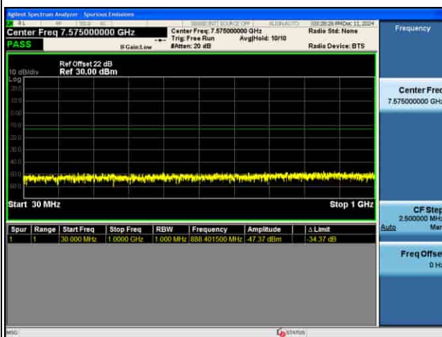
CSE_MIMO(ANT5)_n77(K)_30KHz_64QAM_10M CH630334_1RB@1_
