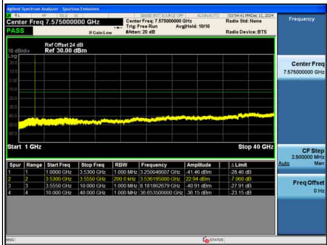
CSE_MIMO(ANT5)_n77(K)_30KHz_16QAM_20M CH630668_1RB@1_
