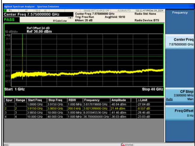
CSE_5G_n77(N)_30KHz_256QAM_60M CH663332_1RB@1_
