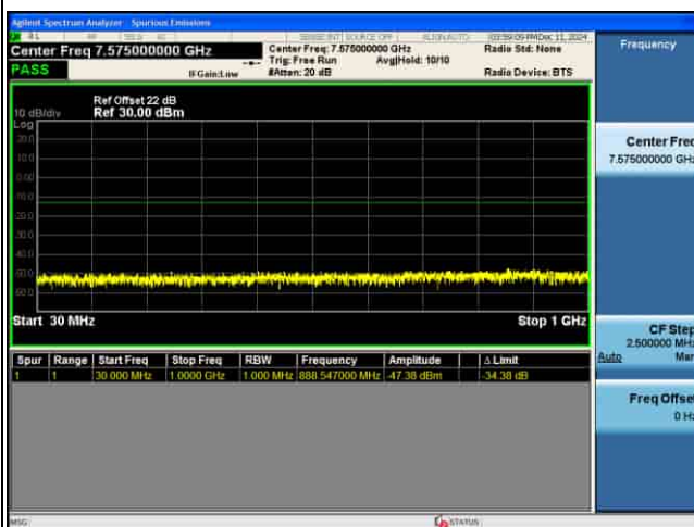
CSE_MIMO(ANT5)_n77(K)_30KHz_64QAM_15M CH630500_1RB@1_
