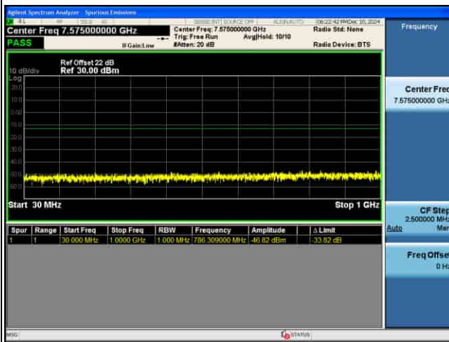
CSE_MIMO(ANT5)_n77(K)_30KHz_16QAM_10M CH630334_1RB@1
