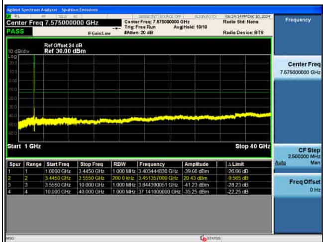
CSE_MIMO(ANT5)_n77(K)_30KHz_64QAM_10M CH630334_1RB@1_
