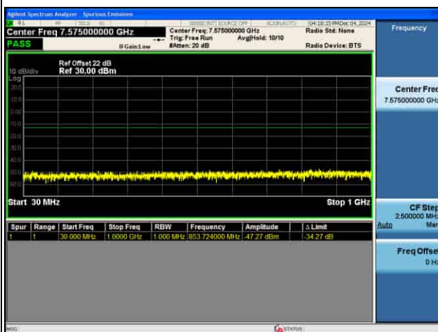
CSE_5G_n77(N)_30KHz_64QAM_80M CH662666_1RB@1
