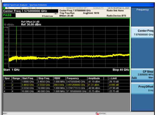
CSE_MIMO(ANT5)_n77(K)_30KHz_QPSK_60M CH634666_1RB@1_
