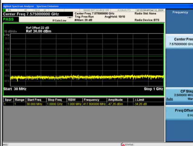
CSE_MIMO(ANT5)_n77(K)_30KHz_16QAM_70M CH633334_1RB@1_
