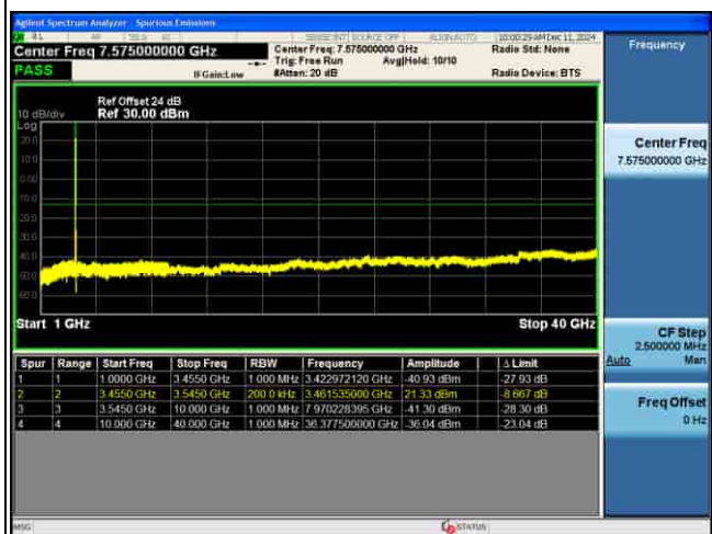
CSE_MIMO(ANT5)_n77(K)_30KHz_16QAM_80M CH633334_1RB@1_
