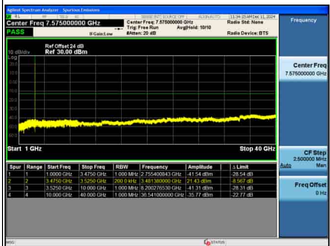
CSE_MIMO(ANT5)_n77(K)_30KHz_QPSK_40M CH635332_1RB@1_
