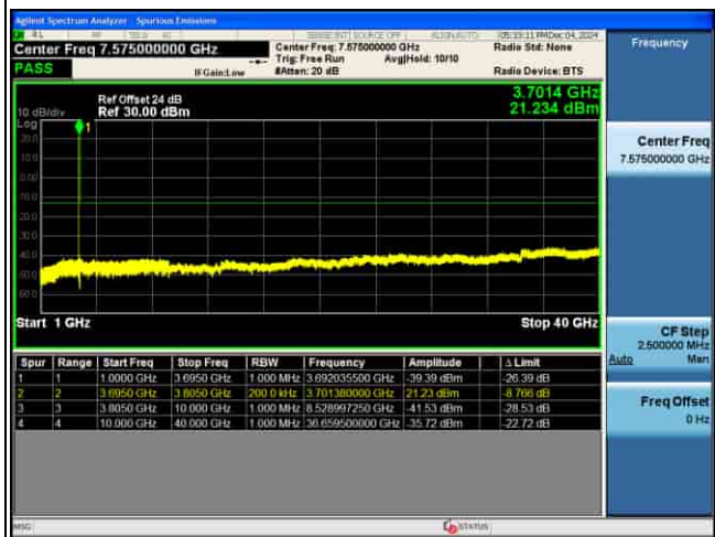
CSE_5G_n77(N)_30KHz_64QAM_100M CH656000_1RB@1_
