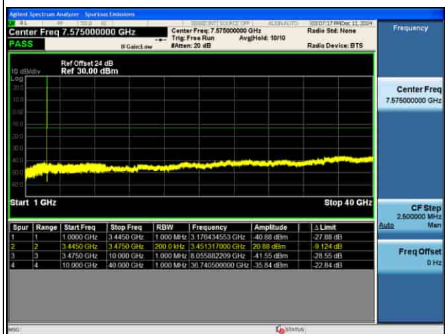
CSE_MIMO(ANT5)_n77(K)_30KHz_64QAM_20M CH630668_1RB@1_
