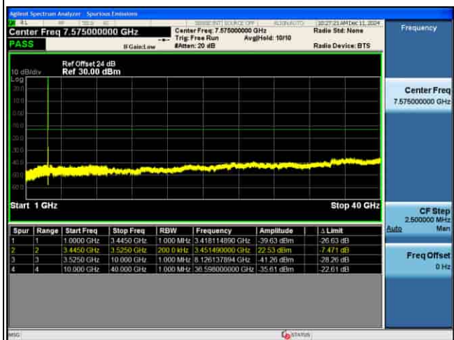
CSE_MIMO(ANT5)_n77(K)_30KHz_16QAM_70M CH633334_1RB@1_
