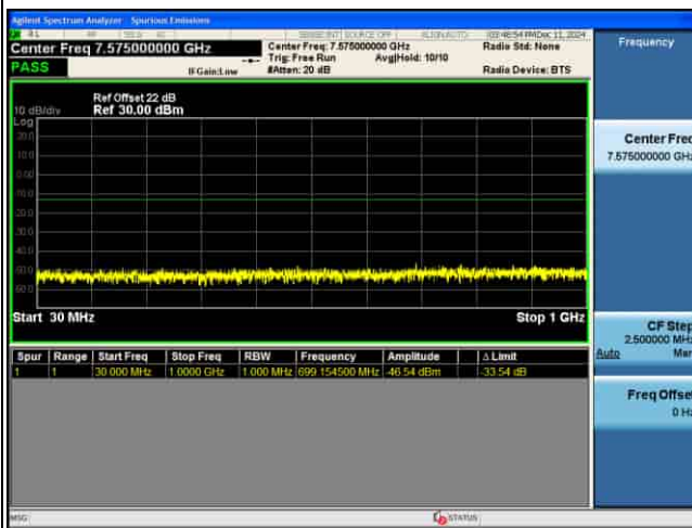
CSE_MIMO(ANT5)_n77(K)_30KHz_QPSK_15M CH633334_1RB@1_
