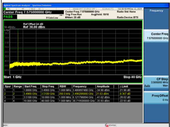
CSE_MIMO(ANT5)_n77(K)_30KHz_16QAM_10M CH633334_1RB@1_
