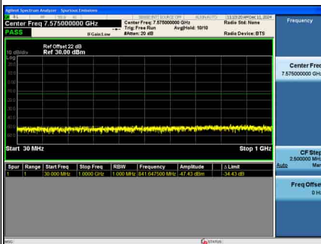
CSE_MIMO(ANT5)_n77(K)_30KHz_16QAM_50M CH633334_1RB@1_
