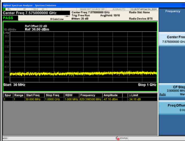
CSE_5G_n77(N)_30KHz_256QAM_30M CH656000_1RB@1_
