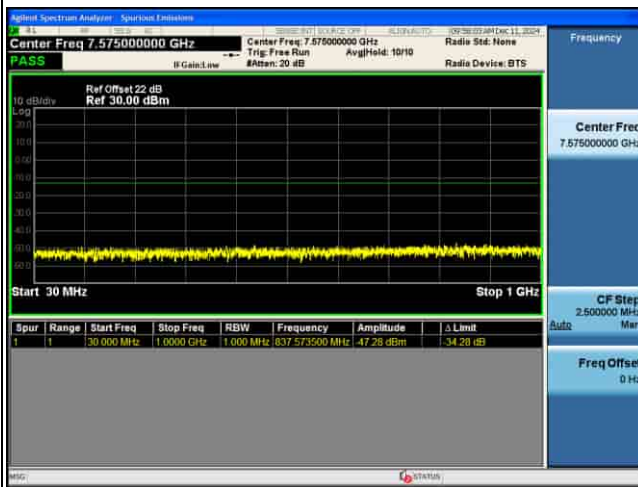
CSE_MIMO(ANT5)_n77(K)_30KHz_16QAM_90M CH633000_1RB@1_
