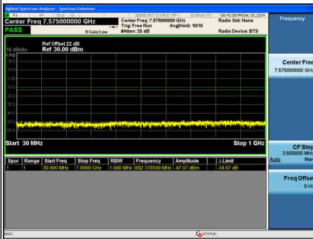
CSE_MIMO(ANT5)_n77(K)_30KHz_16QAM_100M CH633334_1RB@1_
