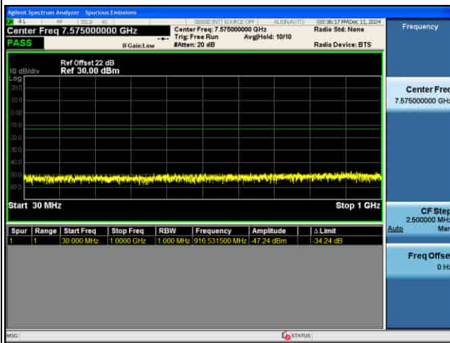
CSE_MIMO(ANT5)_n77(K)_30KHz_16QAM_15M CH630500_1RB@1_
