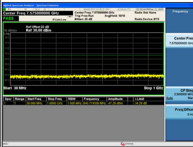
CSE_MIMO(ANT5)_n77(K)_30KHz_16QAM_40M CH631334_1RB@1_
