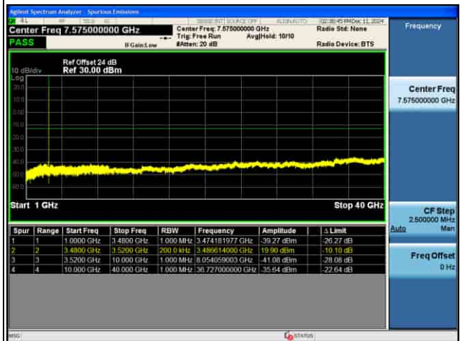
CSE_MIMO(ANT5)_n77(K)_30KHz_QPSK_30M CH635666_1RB@1_
