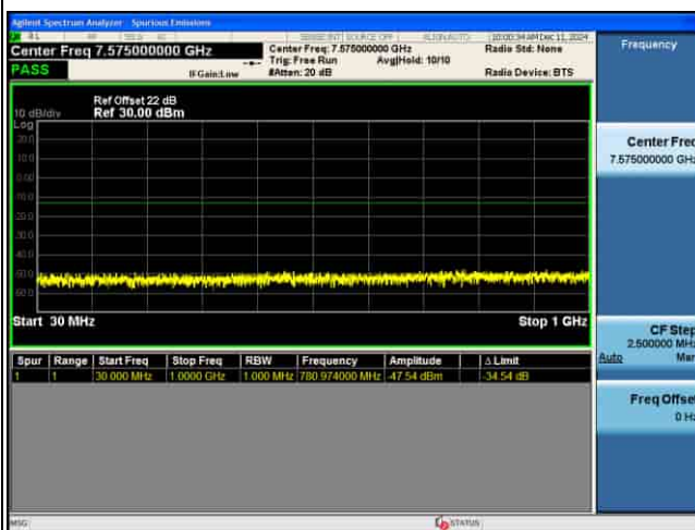
CSE_MIMO(ANT5)_n77(K)_30KHz_16QAM_80M CH633334_1RB@1_
