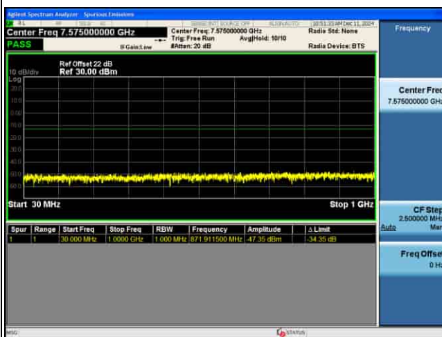
CSE_MIMO(ANT5)_n77(K)_30KHz_64QAM_60M CH632000_1RB@1_
