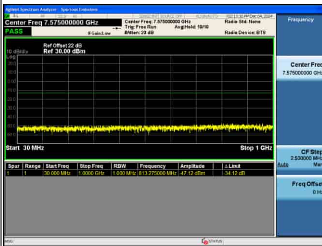
CSE_5G_n77(N)_30KHz_256QAM_40M CH656000_1RB@1_
