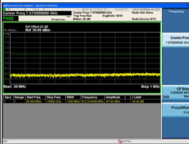
CSE_5G_n77(N)_30KHz_256QAM_70M CH656000_1RB@1_
