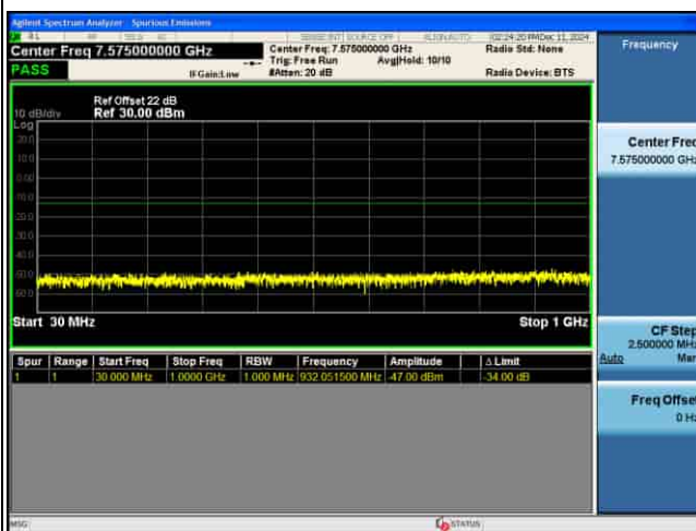
CSE_MIMO(ANT5)_n77(K)_30KHz_64QAM_30M CH631000_1RB@1_
