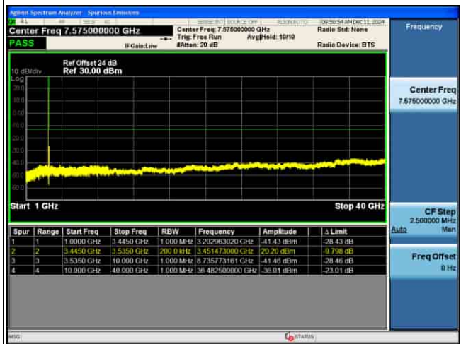
CSE_MIMO(ANT5)_n77(K)_30KHz_QPSK_80M CH633334_1RB@1_
