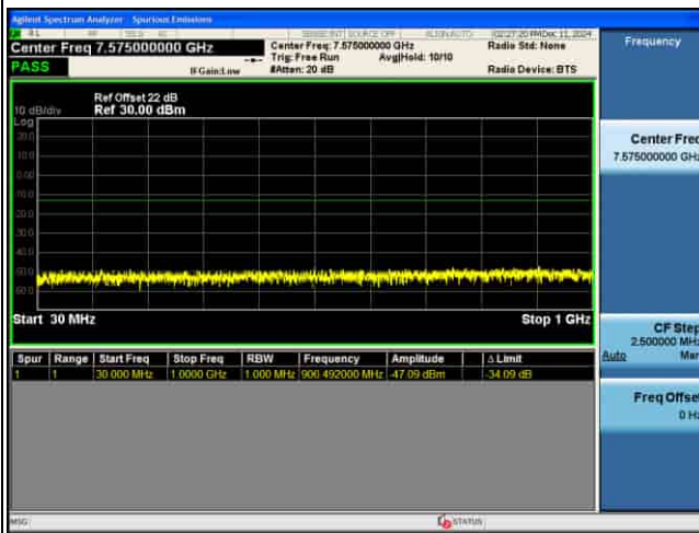
CSE_MIMO(ANT5)_n77(K)_30KHz_64QAM_30M CH635666_1RB@1_
