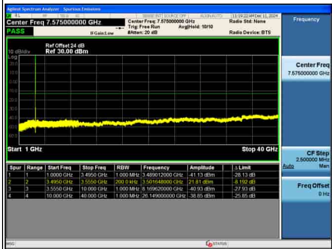
CSE_MIMO(ANT5)_n77(K)_30KHz_16QAM_60M CH632000_1RB@1_
