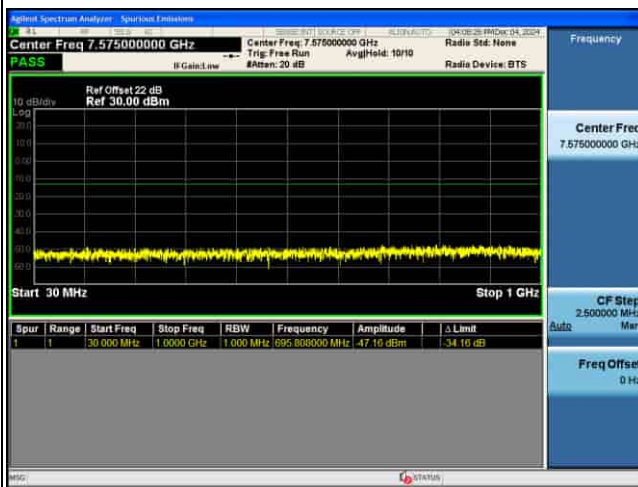
CSE_5G_n77(N)_30KHz_64QAM_80M CH656000_1RB@1
