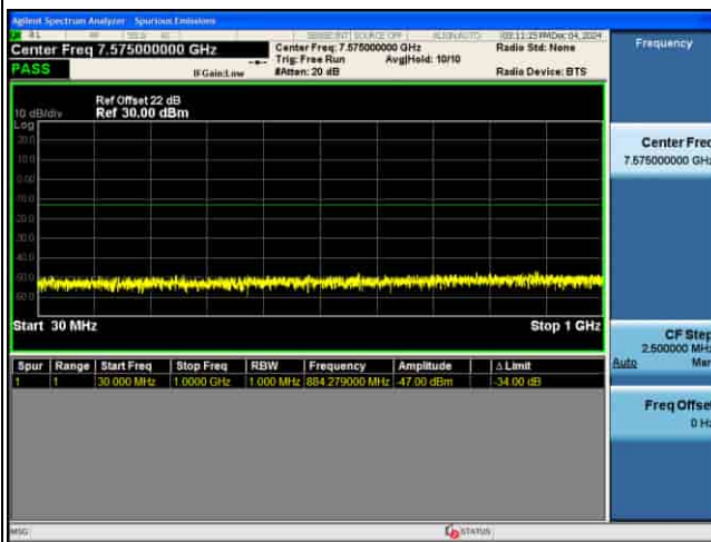
CSE_5G_n77(N)_30KHz_256QAM_60M CH656000_1RB@1_
