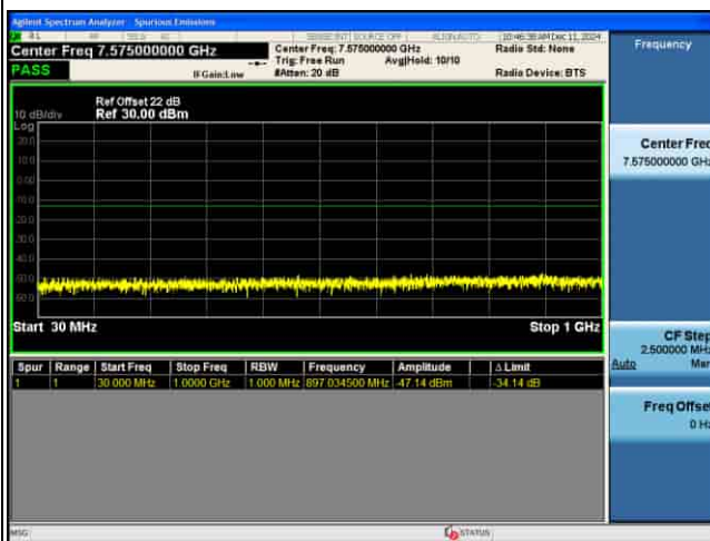
CSE_MIMO(ANT5)_n77(K)_30KHz_16QAM_60M CH633334_1RB@1_
