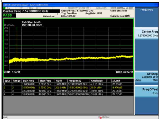
CSE_MIMO(ANT5)_n77(K)_30KHz_64QAM_30M CH631000_1RB@1_
