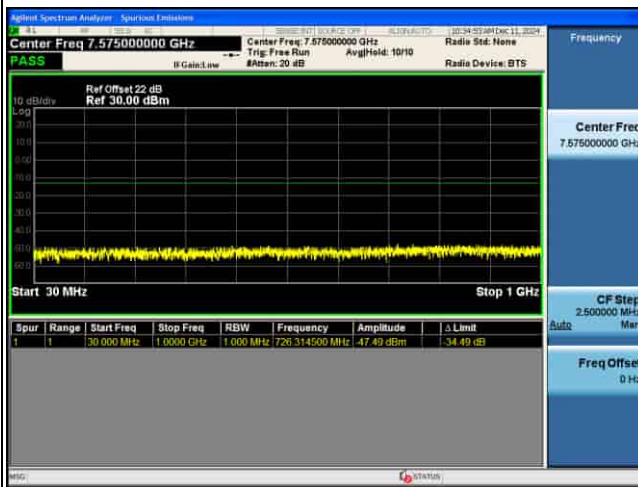
CSE_MIMO(ANT5)_n77(K)_30KHz_QPSK_70M CH633334_1RB@1_
