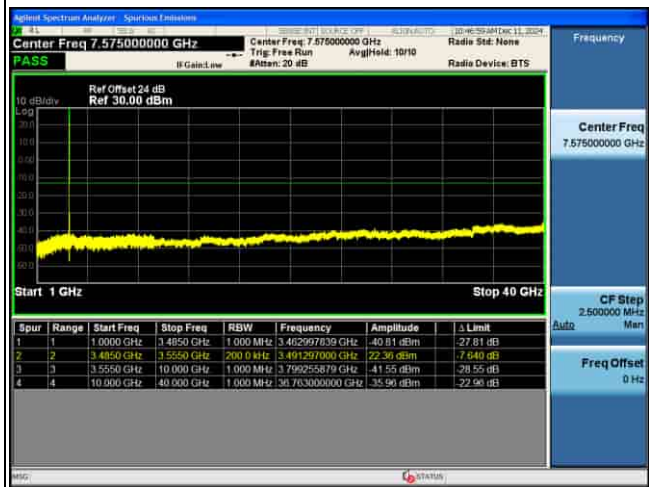
CSE_MIMO(ANT5)_n77(K)_30KHz_16QAM_70M CH632334_1RB@1_
