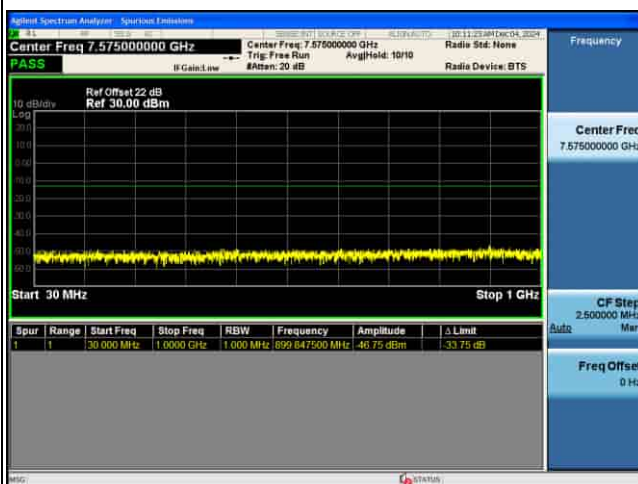
CSE_5G_n77(N)_30KHz_256QAM_10M CH665000_1RB@1_
