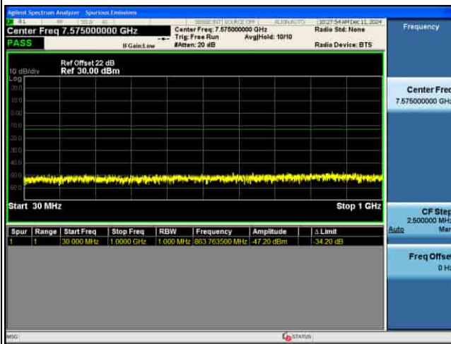
CSE_MIMO(ANT5)_n77(K)_30KHz_16QAM_80M CH632668_1RB@1_
