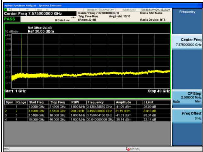
CSE_MIMO(ANT5)_n77(K)_30KHz_64QAM_10M CH636332_1RB@1_
