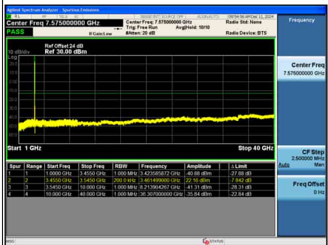
CSE_MIMO(ANT5)_n77(K)_30KHz_QPSK_80M CH634000_1RB@1_
