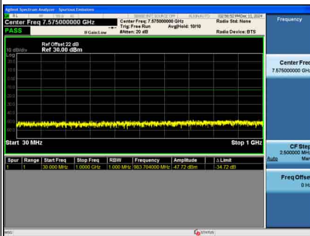
CSE_MIMO(ANT5)_n77(K)_30KHz_16QAM_20M CH633334_1RB@1_
