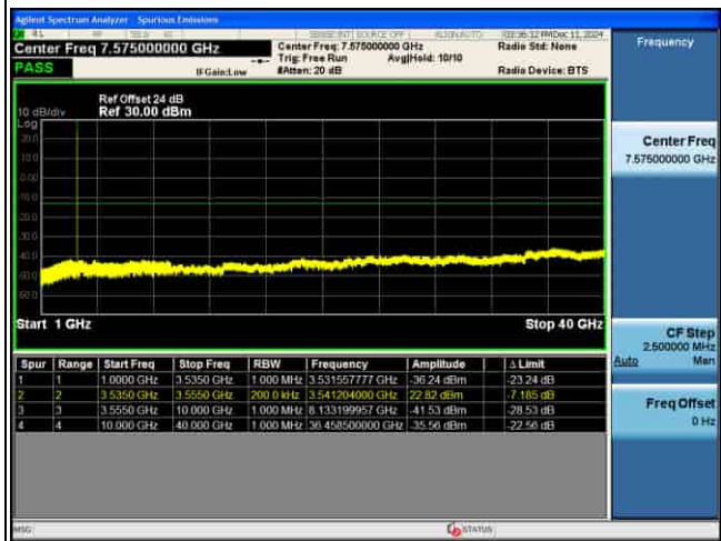
CSE_MIMO(ANT5)_n77(K)_30KHz_16QAM_15M CH630500_1RB@1_
