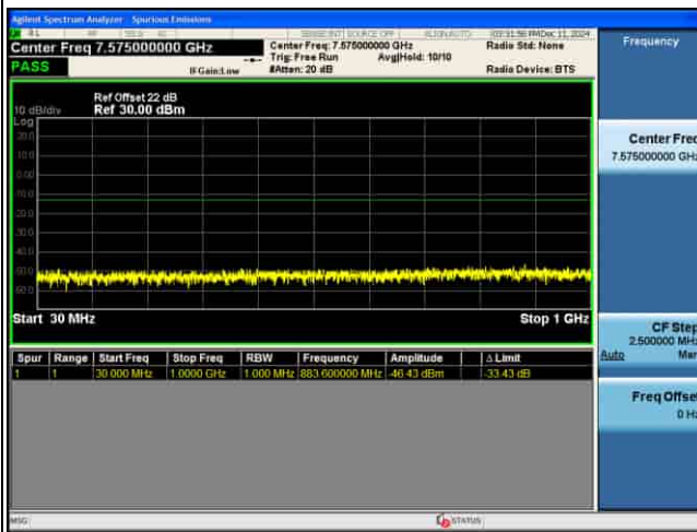
CSE_MIMO(ANT5)_n77(K)_30KHz_64QAM_10M CH636332_1RB@1_
