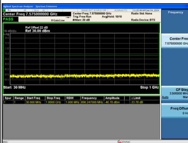
CSE_5G_n77(N)_30KHz_256QAM_20M CH664666_1RB@1_
