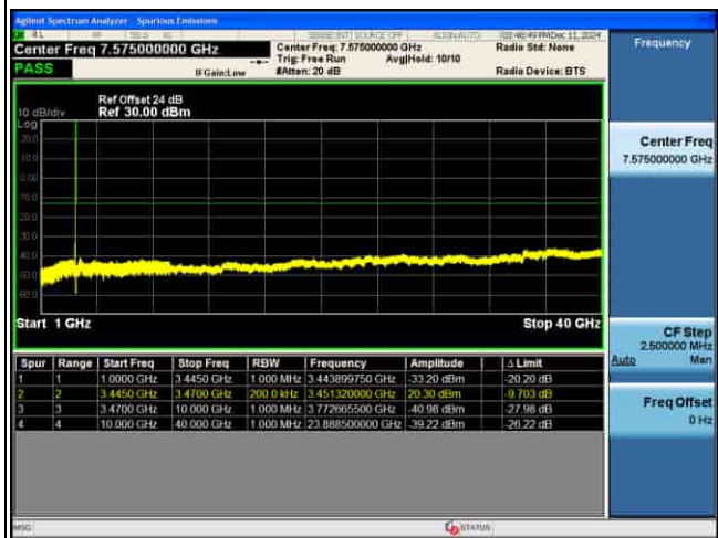
CSE_MIMO(ANT5)_n77(K)_30KHz_QPSK_15M CH633334_1RB@1_
