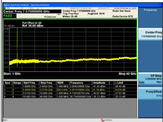
CSE_MIMO(ANT5)_n77(K)_30KHz_16QAM_60M CH633334_1RB@1_
