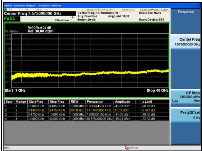
CSE_MIMO(ANT5)_n77(K)_30KHz_QPSK_20M CH633334_1RB@1_
