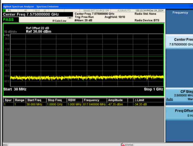
CSE_5G_n77(N)_30KHz_64QAM_100M CH662000_1RB@1_
