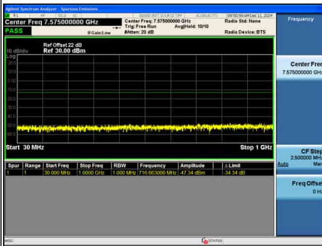
CSE_MIMO(ANT5)_n77(K)_30KHz_QPSK_80M CH633334_1RB@1_
