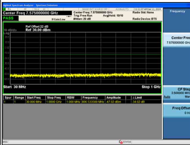
CSE_MIMO(ANT5)_n77(K)_30KHz_64QAM_50M CH635000_1RB@1_
