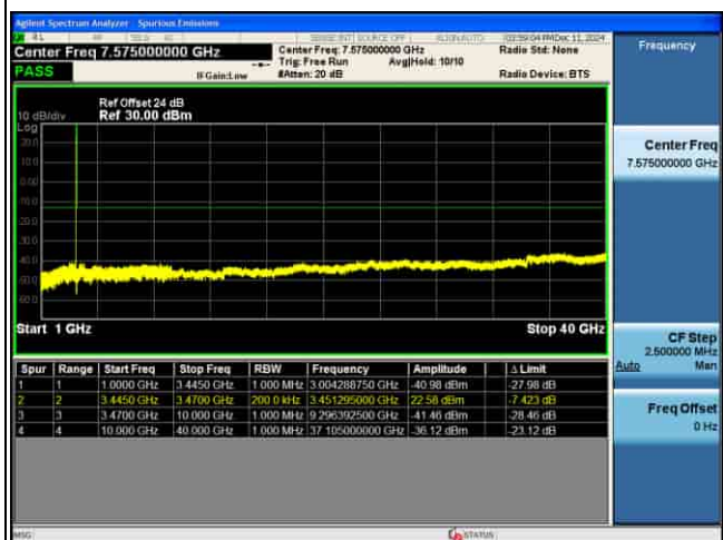
CSE_MIMO(ANT5)_n77(K)_30KHz_64QAM_15M CH630500_1RB@1_
