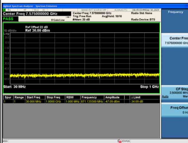
CSE_MIMO(ANT5)_n77(K)_30KHz_16QAM_90M CH633334_1RB@1_
