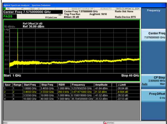
CSE_MIMO(ANT5)_n77(K)_30KHz_QPSK_80M CH634000_1RB@1_
