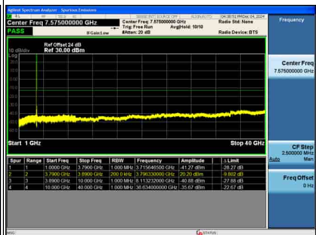
CSE_5G_n77(N)_30KHz_64QAM_90M CH662332_1RB@1_
