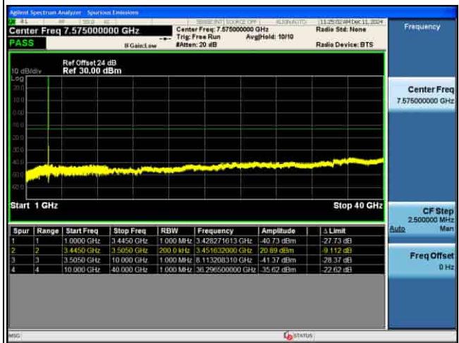
CSE_MIMO(ANT5)_n77(K)_30KHz_QPSK_50M CH633334_1RB@1_
