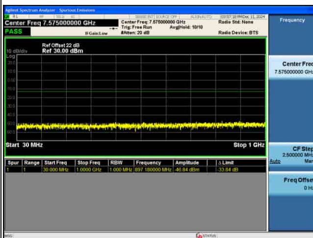
CSE_MIMO(ANT5)_n77(K)_30KHz_16QAM_15M CH633334_1RB@1_
