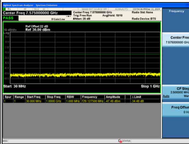
CSE_MIMO(ANT5)_n77(K)_30KHz_16QAM_20M CH630668_1RB@1_
