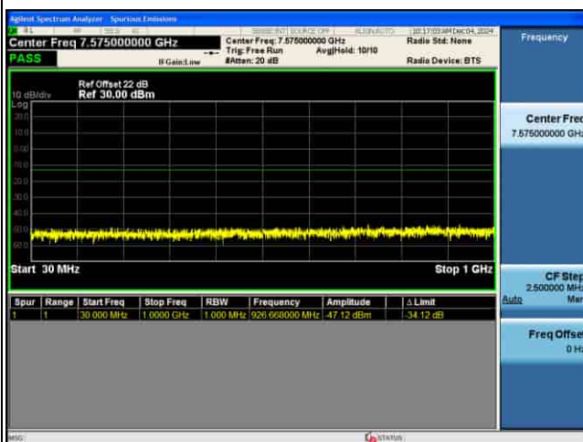
CSE_5G_n77(N)_30KHz_256QAM_15M CH664832_1RB@1_
