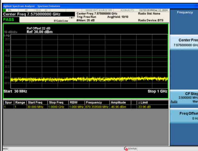
CSE_MIMO(ANT5)_n77(K)_30KHz_QPSK_20M CH636000_1RB@1_
