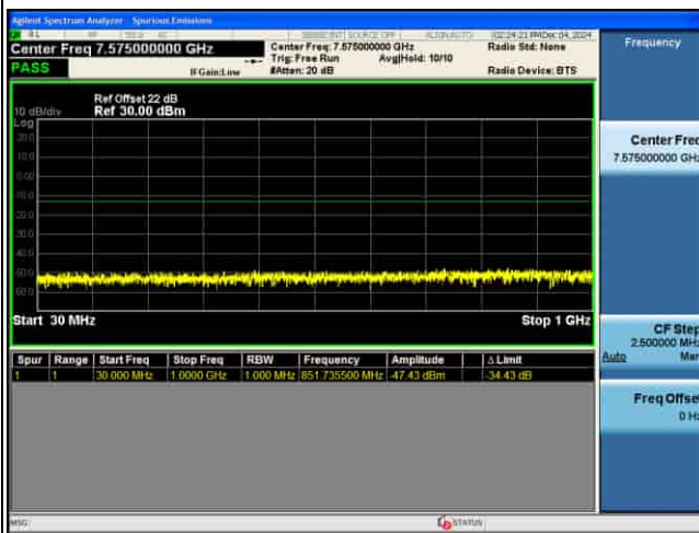
CSE_5G_n77(N)_30KHz_256QAM_50M CH656000_1RB@1_
