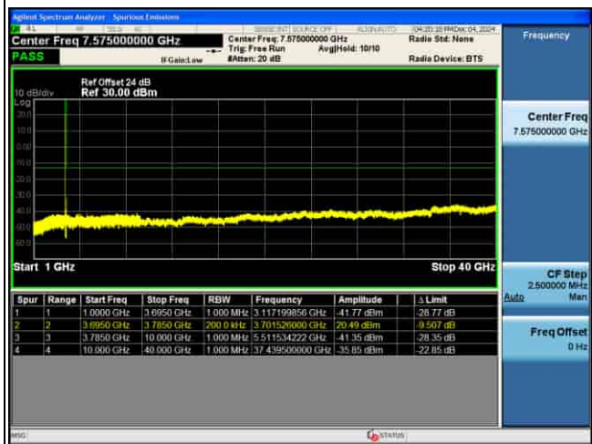
CSE_5G_n77(N)_30KHz_256QAM_80M CH656000_1RB@1_
