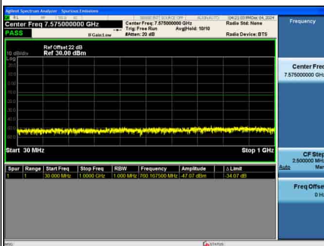
CSE_5G_n77(N)_30KHz_256QAM_80M CH662666_1RB@1_
