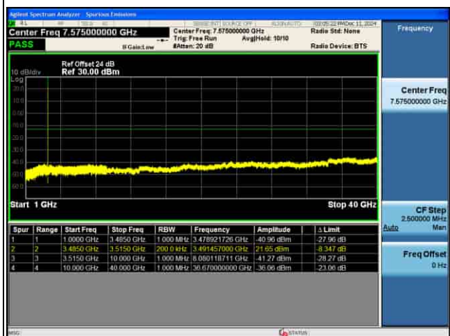
CSE_MIMO(ANT5)_n77(K)_30KHz_16QAM_20M CH633334_1RB@1_
