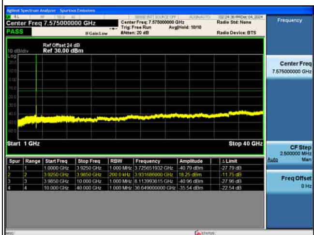
CSE_5G_n77(N)_30KHz_256QAM_50M CH663666_1RB@1_
