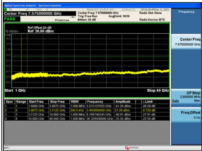
CSE_MIMO(ANT5)_n77(K)_30KHz_64QAM_15M CH636166_1RB@1_
