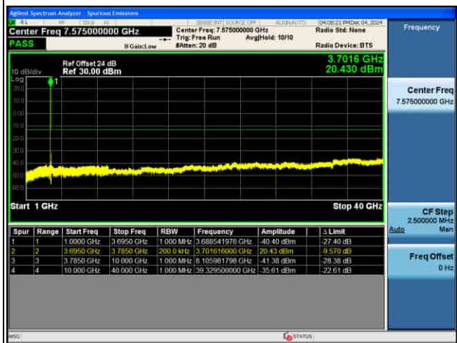
CSE_5G_n77(N)_30KHz_64QAM_80M CH656000_1RB@1_
