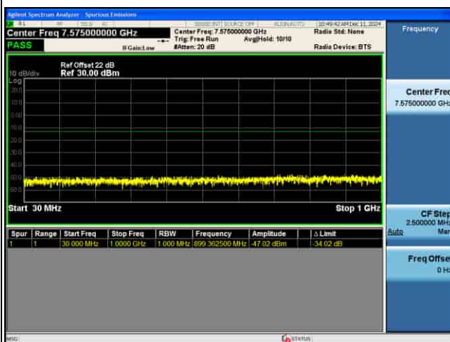
CSE_MIMO(ANT5)_n77(K)_30KHz_16QAM_60M CH633334_1RB@1_
