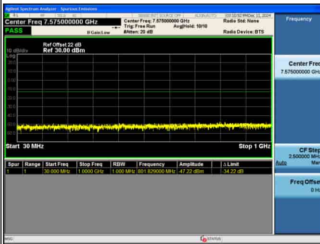
CSE_MIMO(ANT5)_n77(K)_30KHz_64QAM_20M CH636000_1RB@1_
