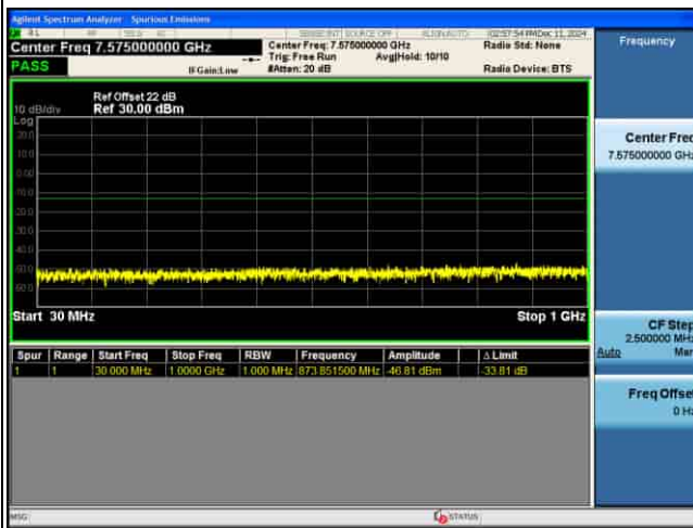
CSE_MIMO(ANT5)_n77(K)_30KHz_16QAM_30M CH631000_1RB@1_
