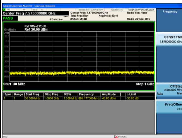
CSE_5G_n77(N)_30KHz_256QAM_60M CH663332_1RB@1_
