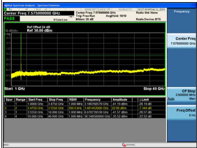
CSE_MIMO(ANT5)_n77(K)_30KHz_16QAM_80M CH632668_1RB@1_
