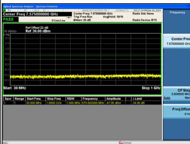
CSE_5G_n77(N)_30KHz_256QAM_70M CH663000_1RB@1_
