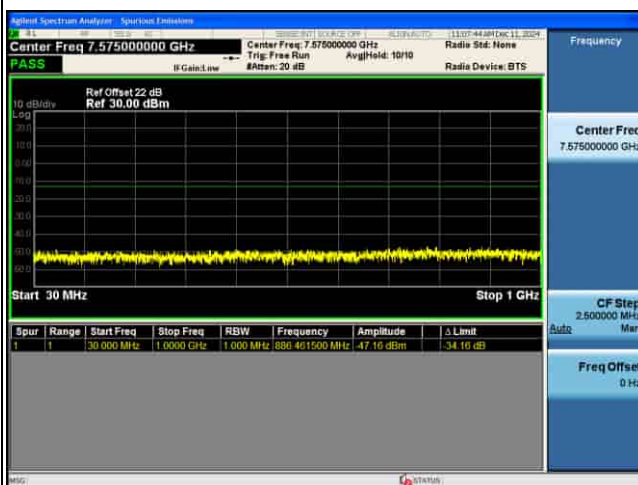
CSE_MIMO(ANT5)_n77(K)_30KHz_64QAM_50M CH631668_1RB@1_
