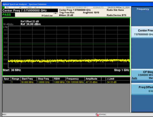
CSE_MIMO(ANT5)_n77(K)_30KHz_64QAM_15M CH636166_1RB@1_
