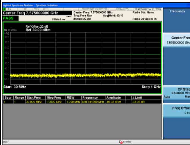
CSE_MIMO(ANT5)_n77(K)_30KHz_16QAM_70M CH632334_1RB@1_
