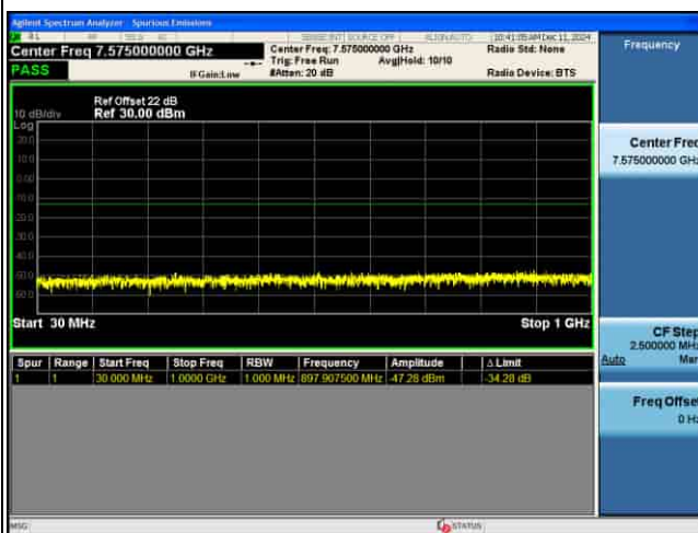
CSE_MIMO(ANT5)_n77(K)_30KHz_QPSK_60M CH634666_1RB@1_
