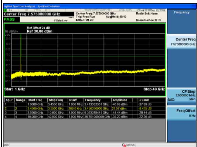
CSE_MIMO(ANT5)_n77(K)_30KHz_16QAM_90M CH633334_1RB@1_
