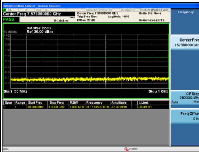
CSE_5G_n77(N)_30KHz_64QAM_90M CH656000_1RB@1_
