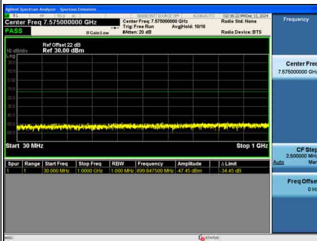
CSE_MIMO(ANT5)_n77(K)_30KHz_QPSK_30M CH635666_1RB@1_
