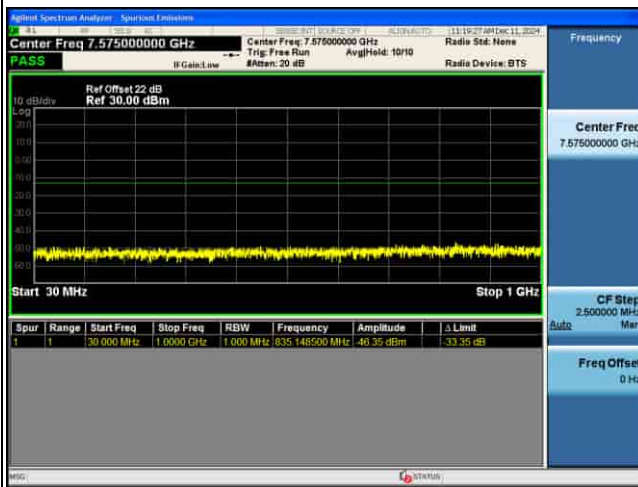
CSE_MIMO(ANT5)_n77(K)_30KHz_16QAM_60M CH632000_1RB@1_
