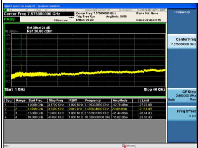
CSE_MIMO(ANT5)_n77(K)_30KHz_QPSK_50M CH635000_1RB@1_
