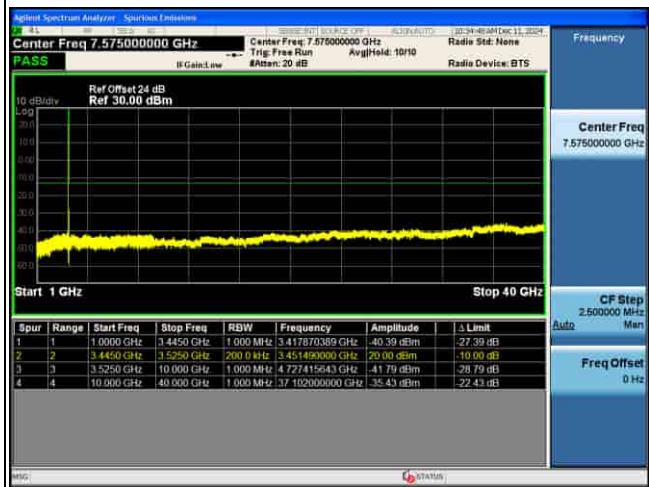
CSE_MIMO(ANT5)_n77(K)_30KHz_QPSK_70M CH633334_1RB@1_
