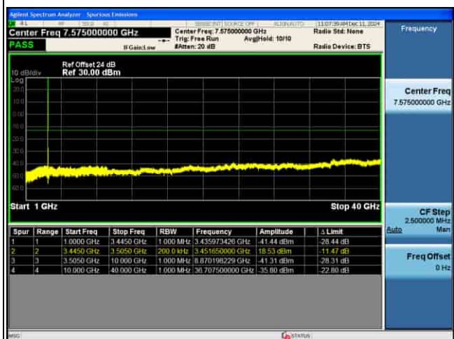
CSE_MIMO(ANT5)_n77(K)_30KHz_64QAM_50M CH631668_1RB@1_
