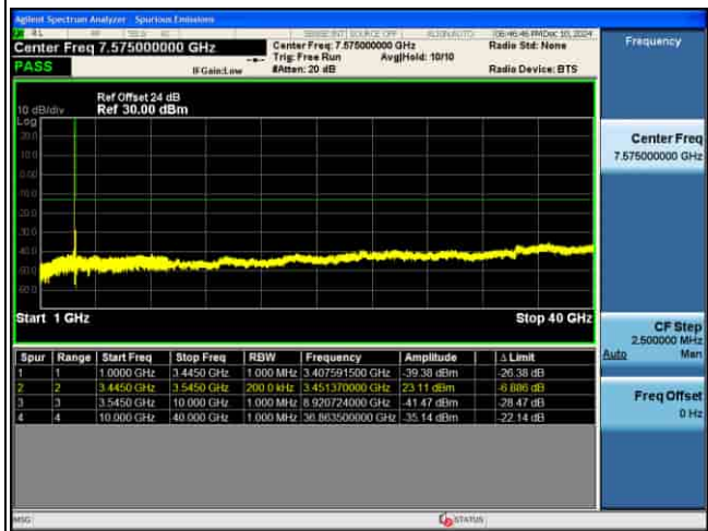
CSE_MIMO(ANT5)_n77(K)_30KHz_QPSK_90M CH633334_1RB@1_
