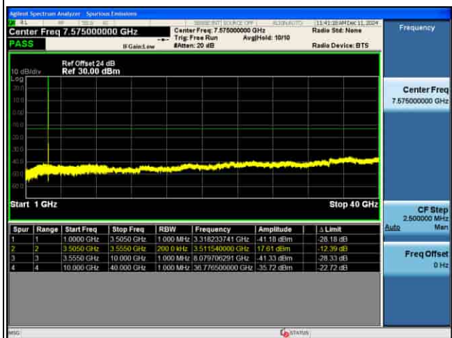
CSE_MIMO(ANT5)_n77(K)_30KHz_64QAM_50M CH631668_1RB@1_
