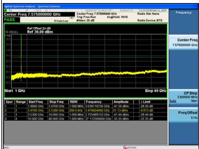
CSE_MIMO(ANT5)_n77(K)_30KHz_16QAM_50M CH633334_1RB@1_
