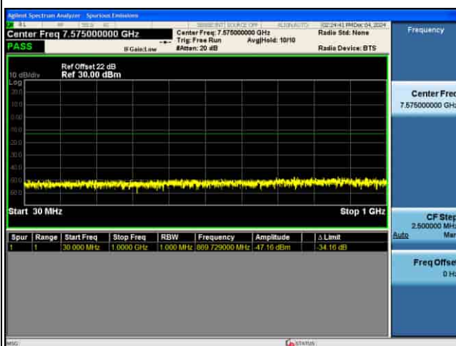
CSE_5G_n77(N)_30KHz_256QAM_50M CH663666_1RB@1_
