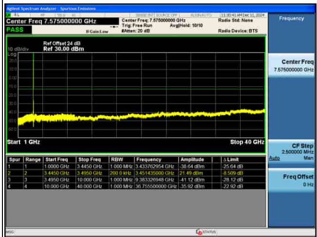
CSE_MIMO(ANT5)_n77(K)_30KHz_QPSK_40M CH633334_1RB@1_
