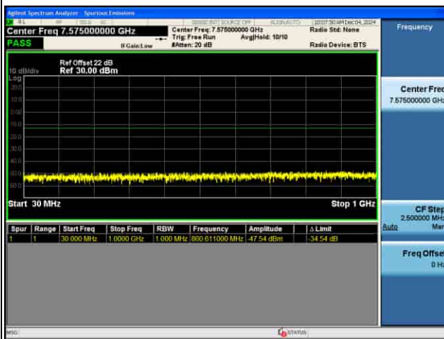
CSE_5G_n77(N)_30KHz_256QAM_10M CH656000_1RB@1_
