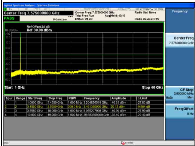
CSE_MIMO(ANT5)_n77(K)_30KHz_16QAM_100M CH633334_1RB@1_
