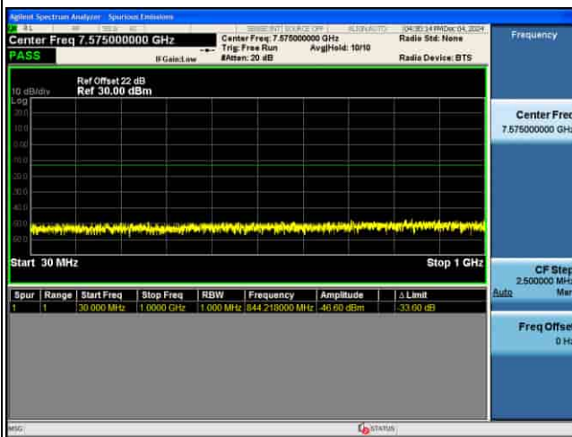
CSE_5G_n77(N)_30KHz_256QAM_90M CH656000_1RB@1_
