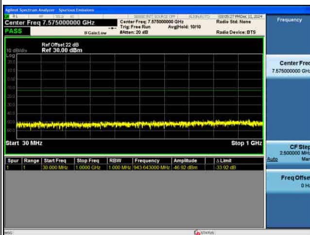
CSE_MIMO(ANT5)_n77(K)_30KHz_16QAM_20M CH633334_1RB@1_
