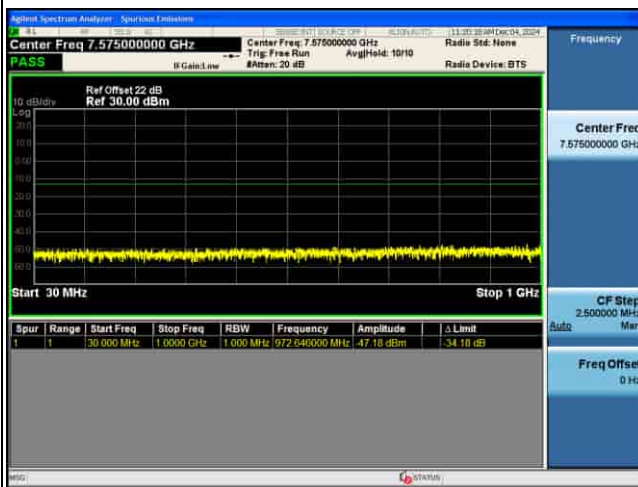
CSE_5G_n77(N)_30KHz_256QAM_20M CH656000_1RB@1_
