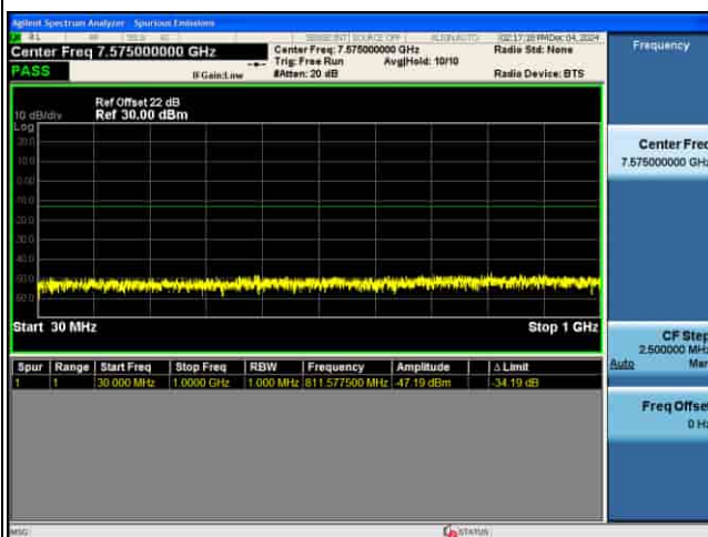
CSE_5G_n77(N)_30KHz_256QAM_40M CH664000_1RB@1_
