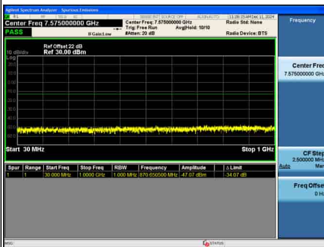
CSE_MIMO(ANT5)_n77(K)_30KHz_QPSK_50M CH635000_1RB@1_
