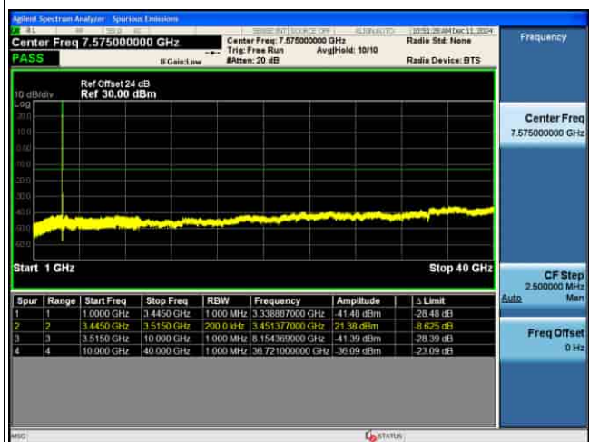
CSE_MIMO(ANT5)_n77(K)_30KHz_64QAM_60M CH632000_1RB@1_
