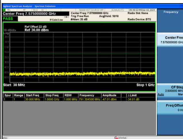
CSE_5G_n77(N)_30KHz_256QAM_100M CH662000_1RB@1
