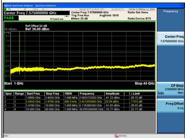
CSE_MIMO(ANT5)_n77(K)_30KHz_16QAM_15M CH633334_1RB@1_
