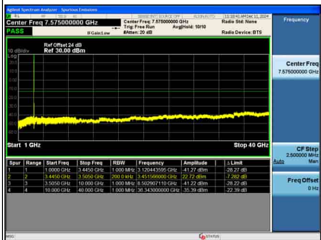
CSE_MIMO(ANT5)_n77(K)_30KHz_16QAM_50M CH633334_1RB@1_
