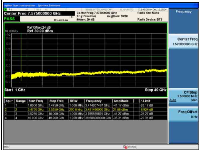
CSE_MIMO(ANT5)_n77(K)_30KHz_64QAM_40M CH635332_1RB@1_
