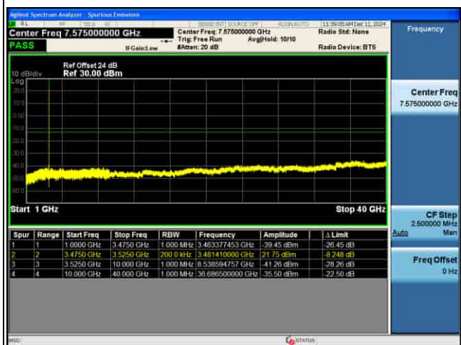
CSE_MIMO(ANT5)_n77(K)_30KHz_16QAM_40M CH633334_1RB@1_
