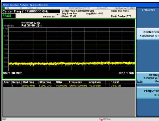
CSE_MIMO(ANT5)_n77(K)_30KHz_16QAM_40M CH633334_1RB@1_
