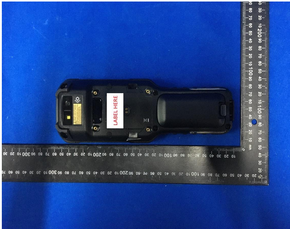
(18) EUT Photoo –S0803 with Alpha Numeric
